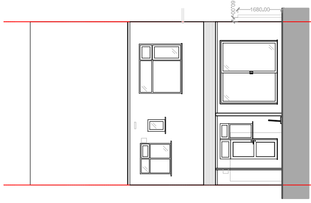
Existing Rear (South) Elevation
