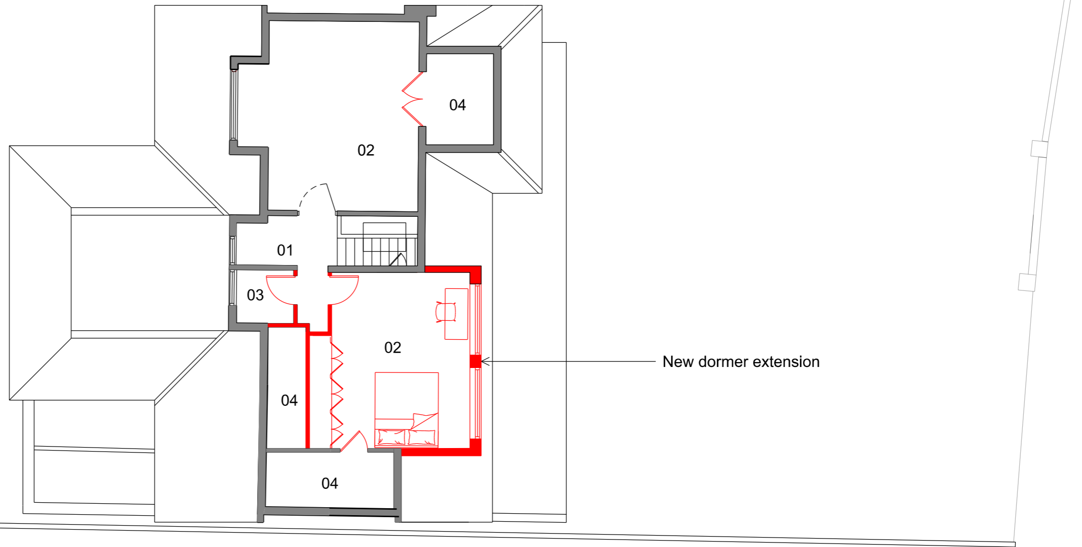
Proposed Second Floor
