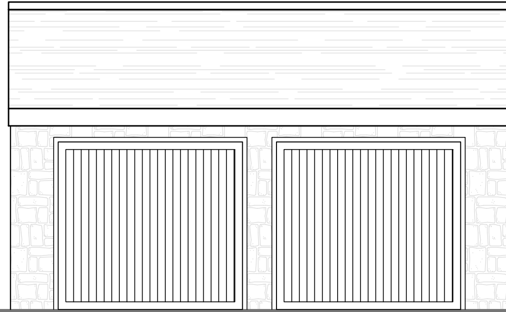
PROPOSED FRONT ELEVATION 1:50
