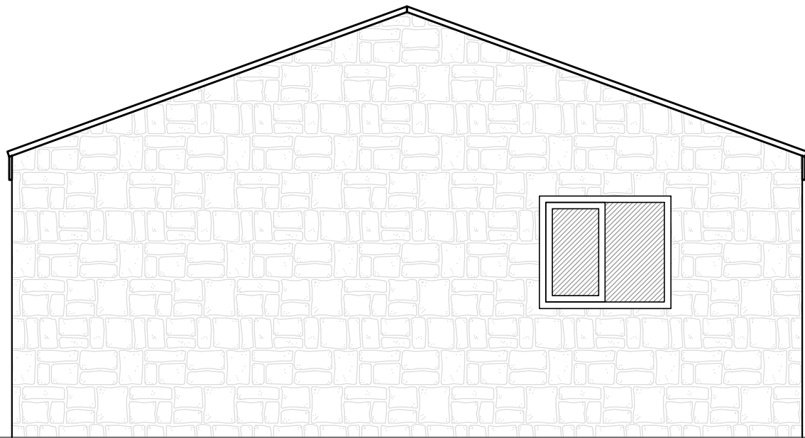
PROPOSED SIDE ELEVATION 1:50
