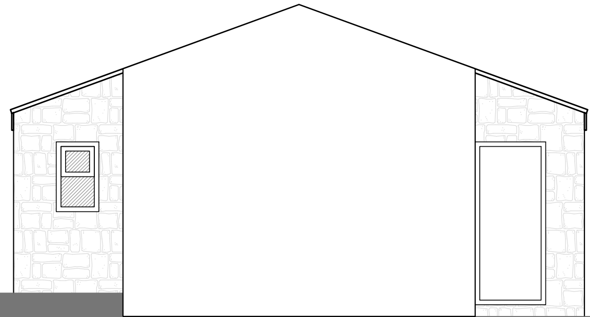
PROPOSED SIDE ELEVATION 1:1:50
