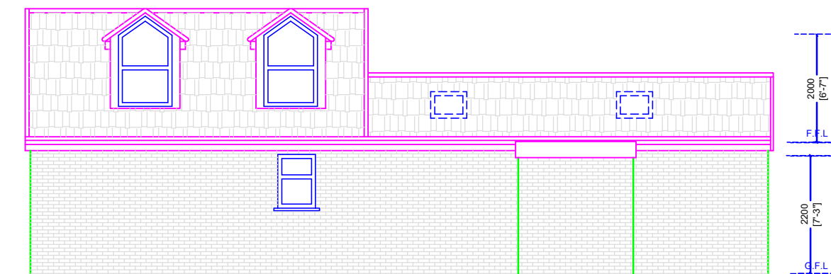
PROPOSED SIDE ELEVATION (NORTH WEST)
