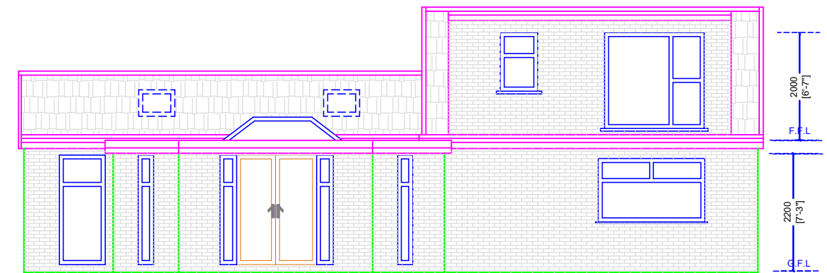
PROPOSED SIDE ELEVATION(SOUTH EAST)
