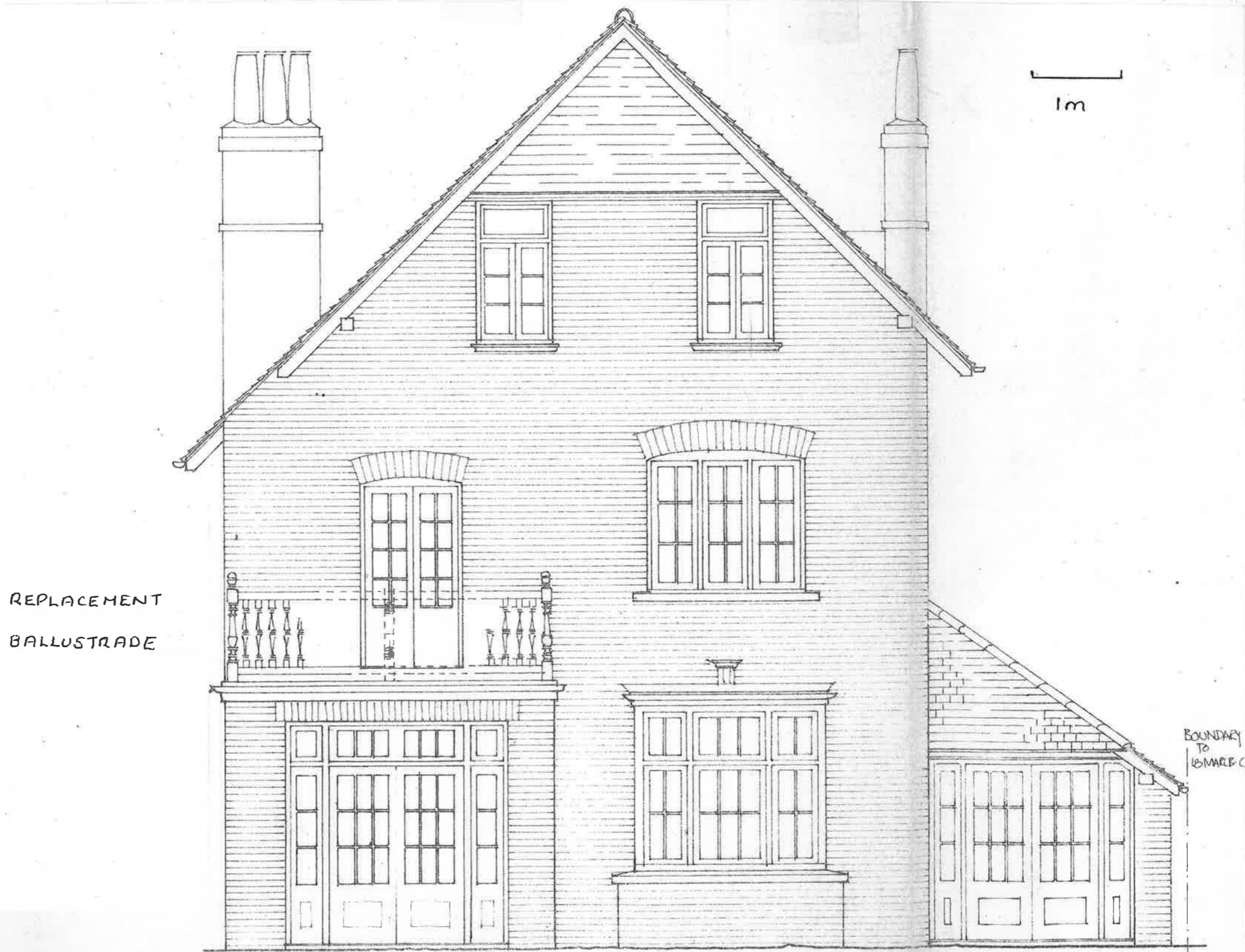
REAR ELEVATION
