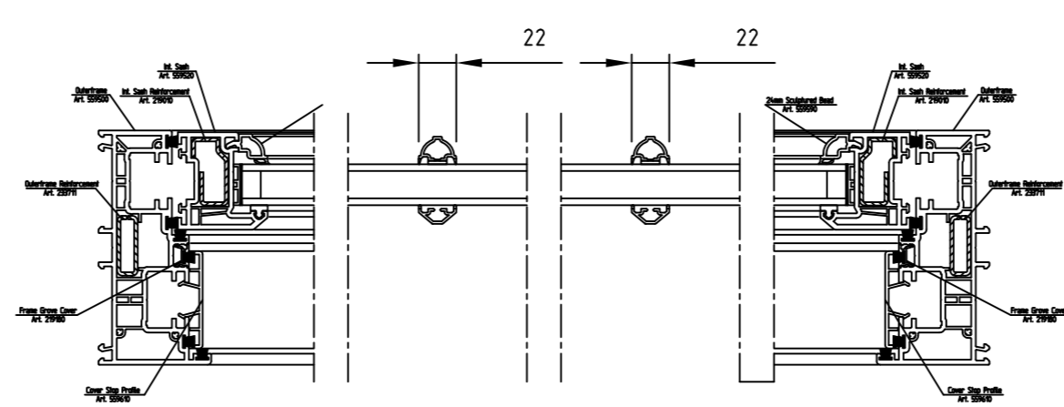
Section C-C
