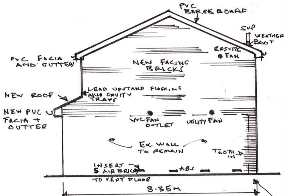
PROPOSED SIDE VIEW 1:100
