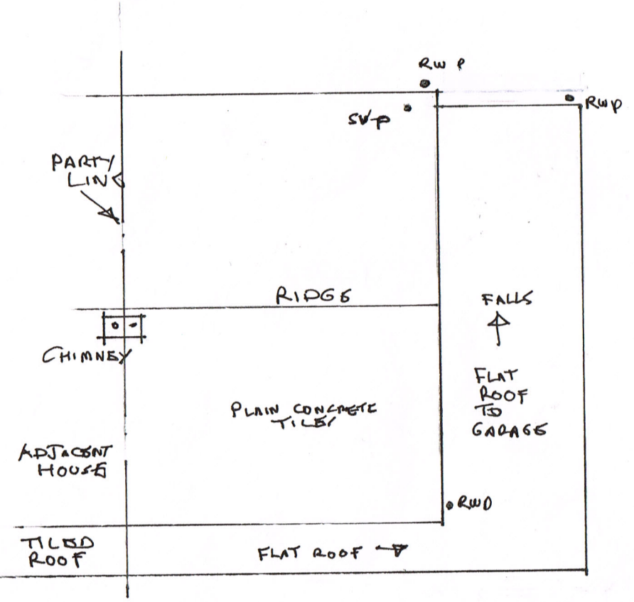
EX. 1:100 ROOF PLAN
