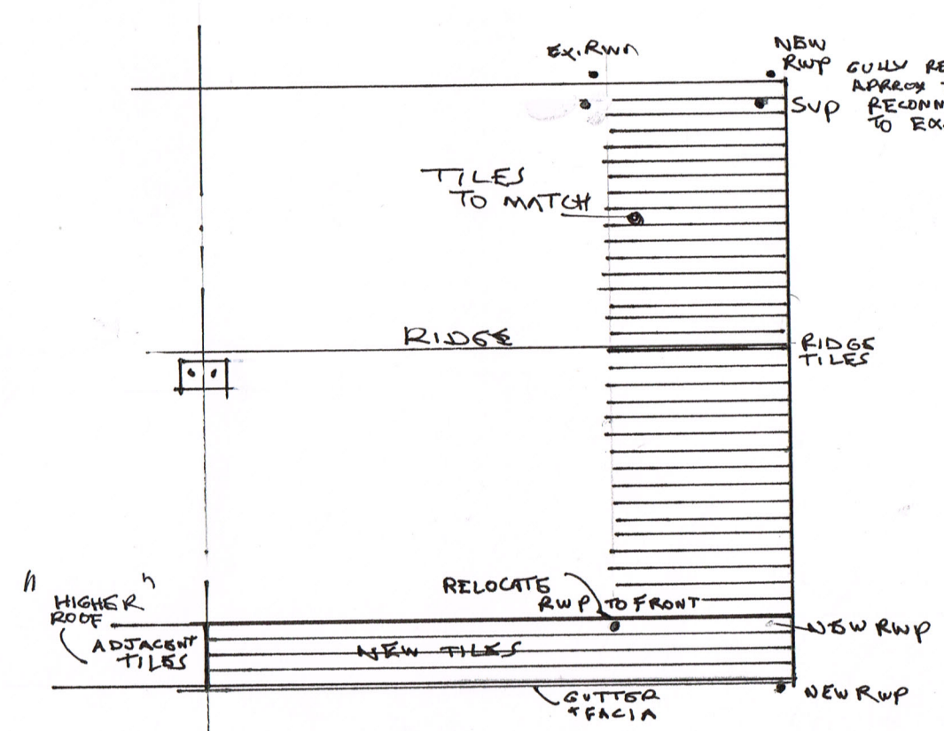
PROPOSED ROOF PLAN 9 MIDDLEHAM ROAD
