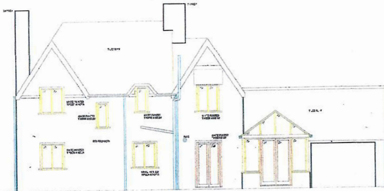
SOUTHEAST ELEVATION
