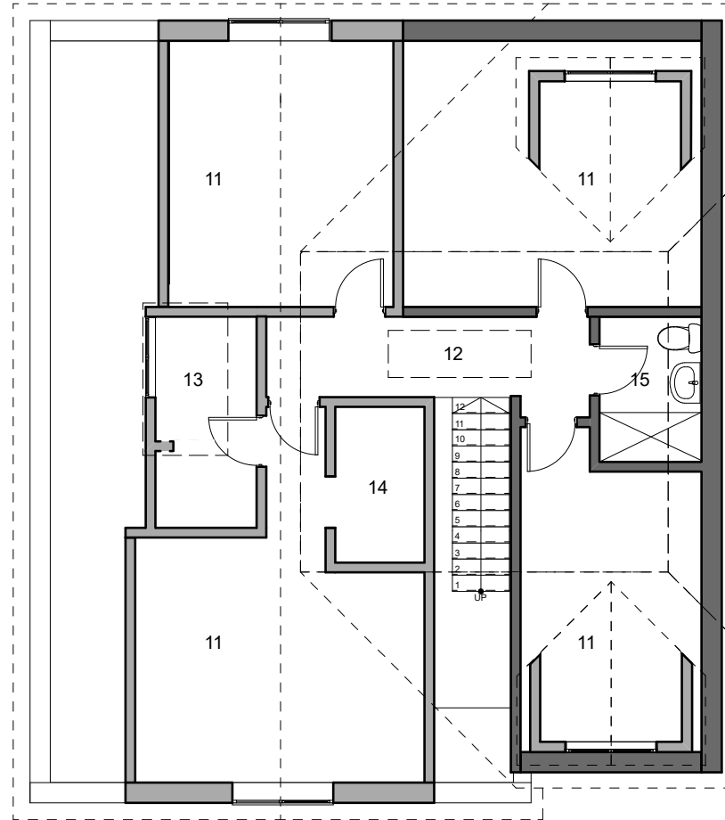
02 PROPOSED FIRST FLOOR Scale 1:100
