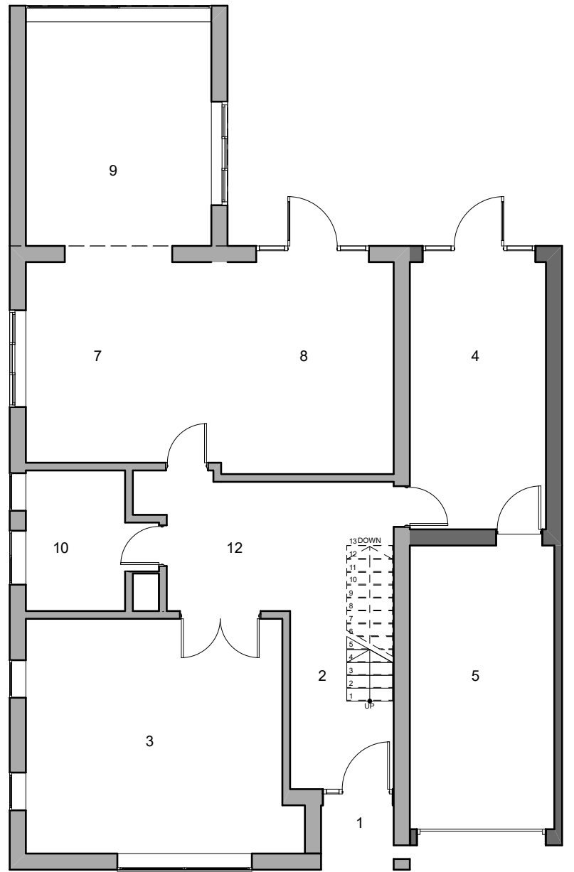
01 PROPOSED GROUND FLOOR Scale 1:100
