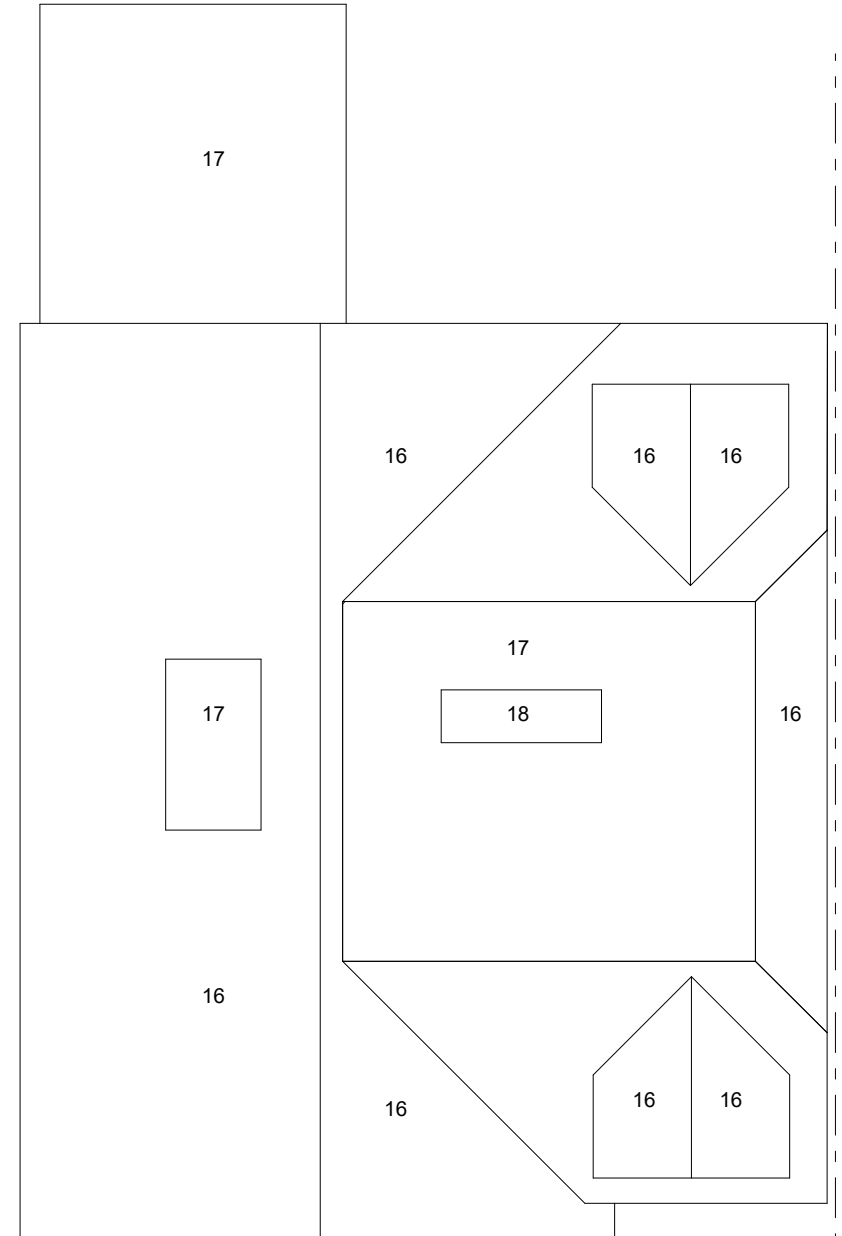
03 PROPOSED ROOF PLAN Scale 1:100
