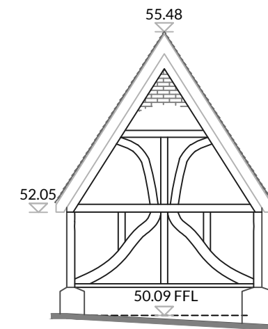
South West Elevation
