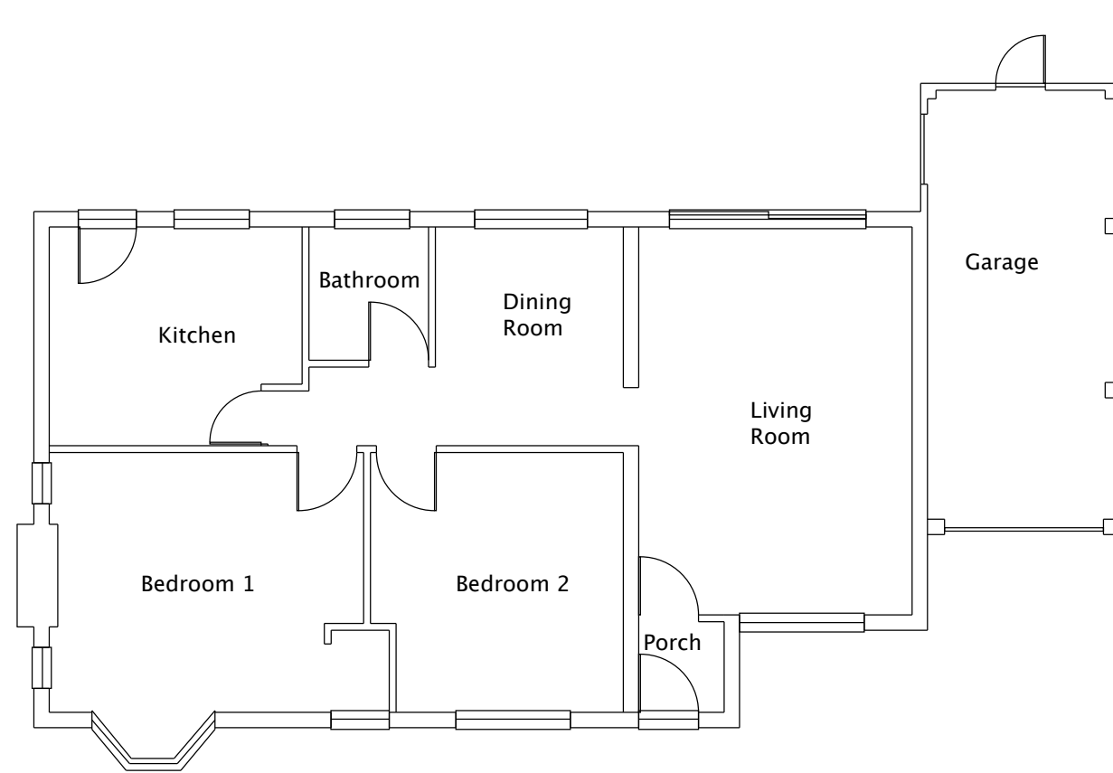
Existing Floorplan
