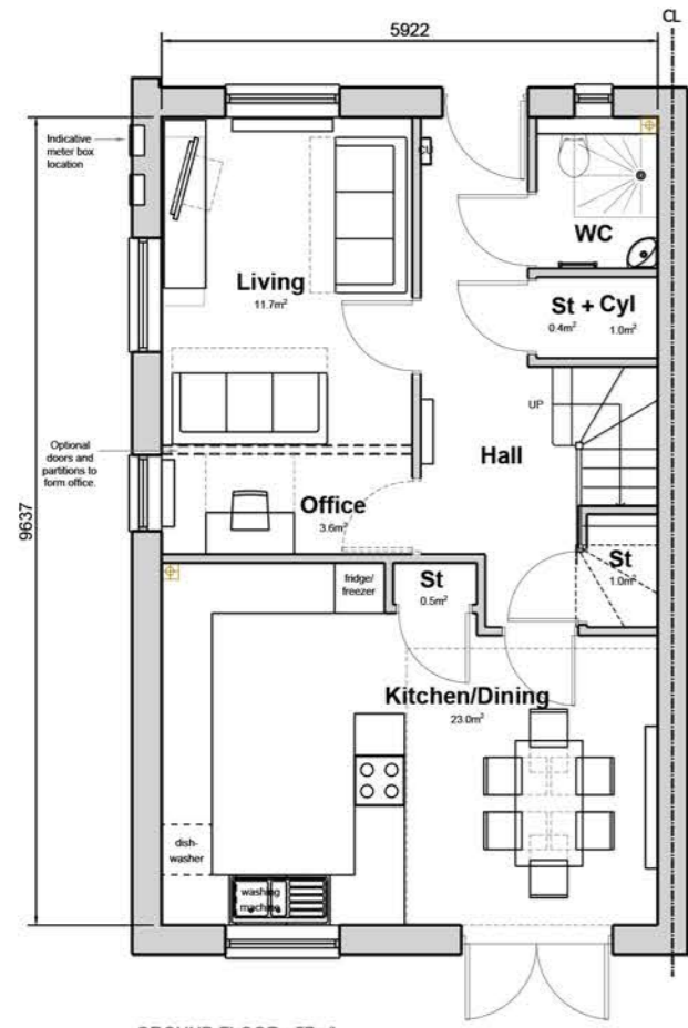
GROUND FLOOR - 57m 2
