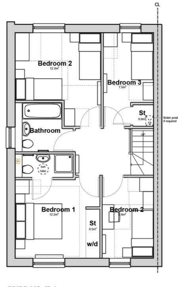
FIRST FLOOR - 57m 2
