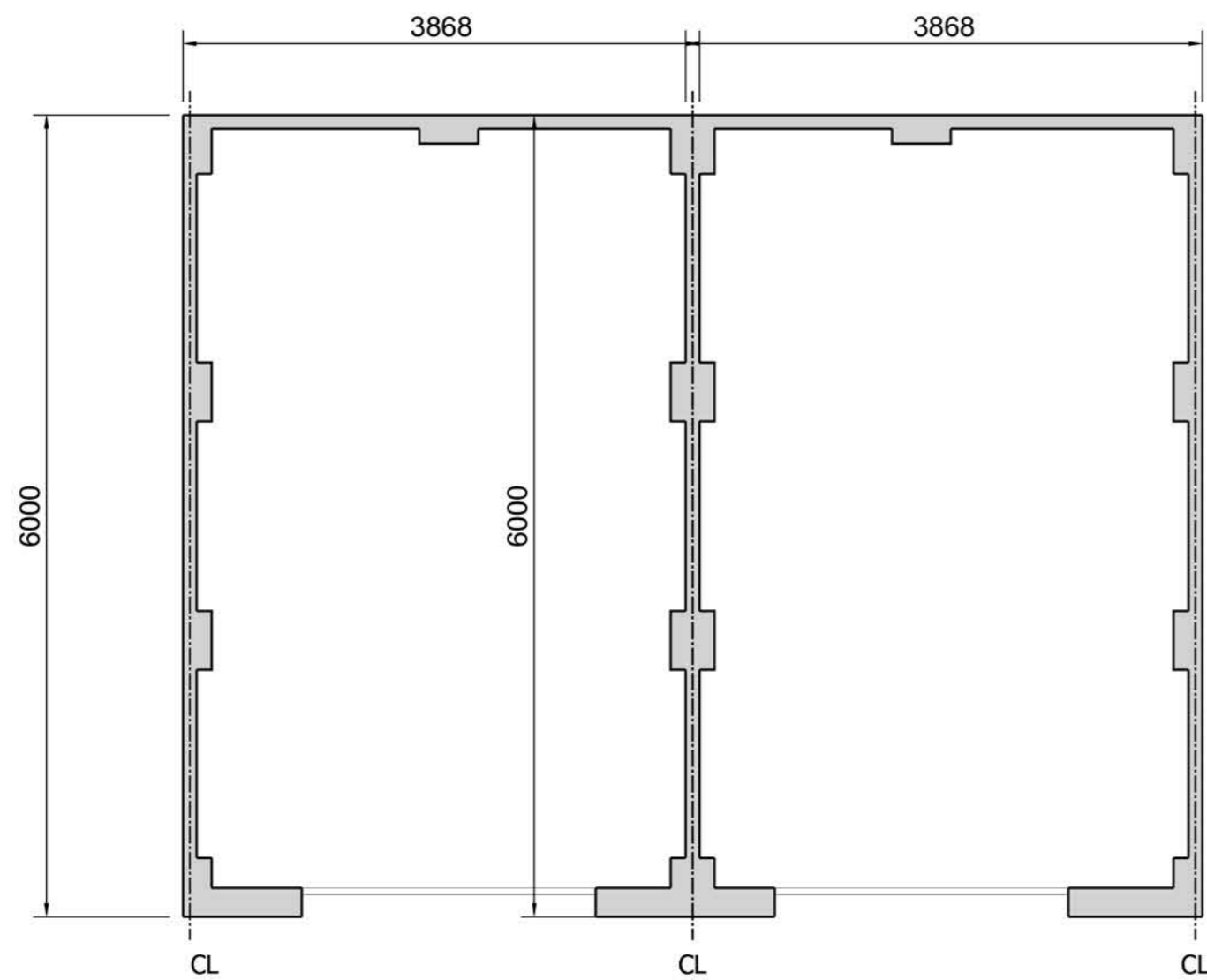
FLOOR PLAN - SINGLE LINK DETACHED GARAGE
