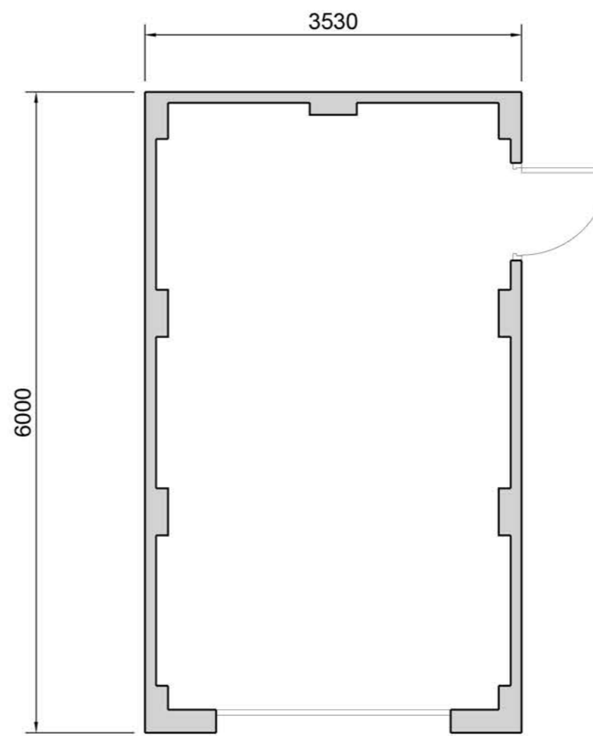
FLOOR PLAN - SINGLE GARAGE
