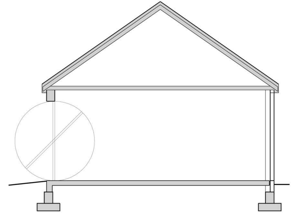
CROSS SECTION
