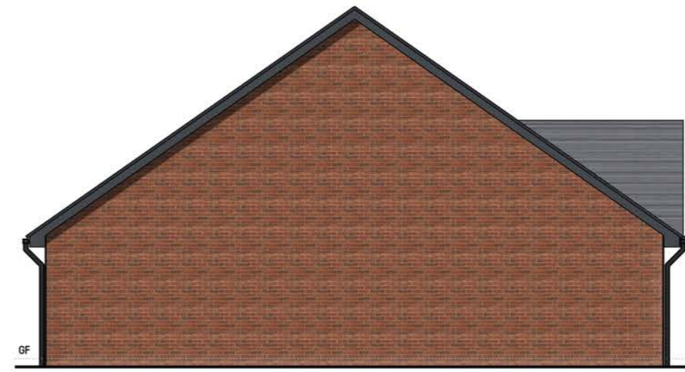
SIDE ELEVATION
