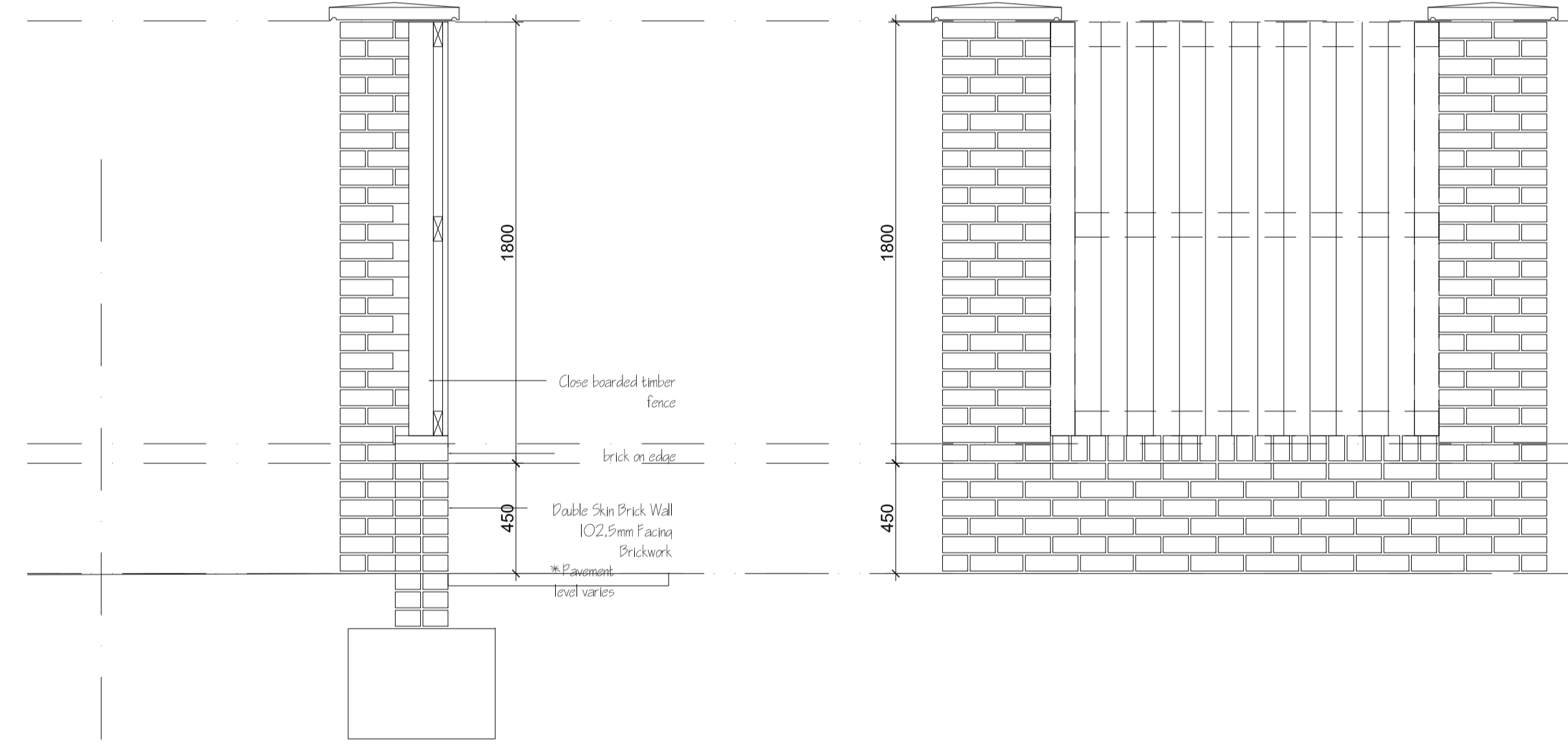
SECTION A-A - BOUNDARY (DWARF WALL + TIMBER FENCE) PLOT 6 SCALE @ 1:20
