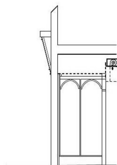
SECTION ON EXISTING SHOPFRONT
