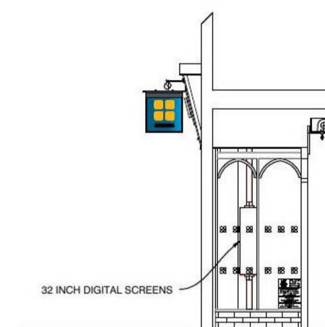
SECTION E-E:
