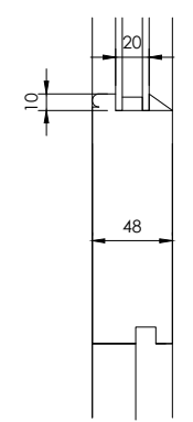
MID RAIL
