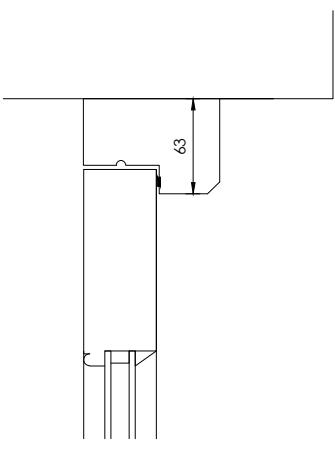
HEAD
