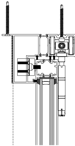
HEAD
