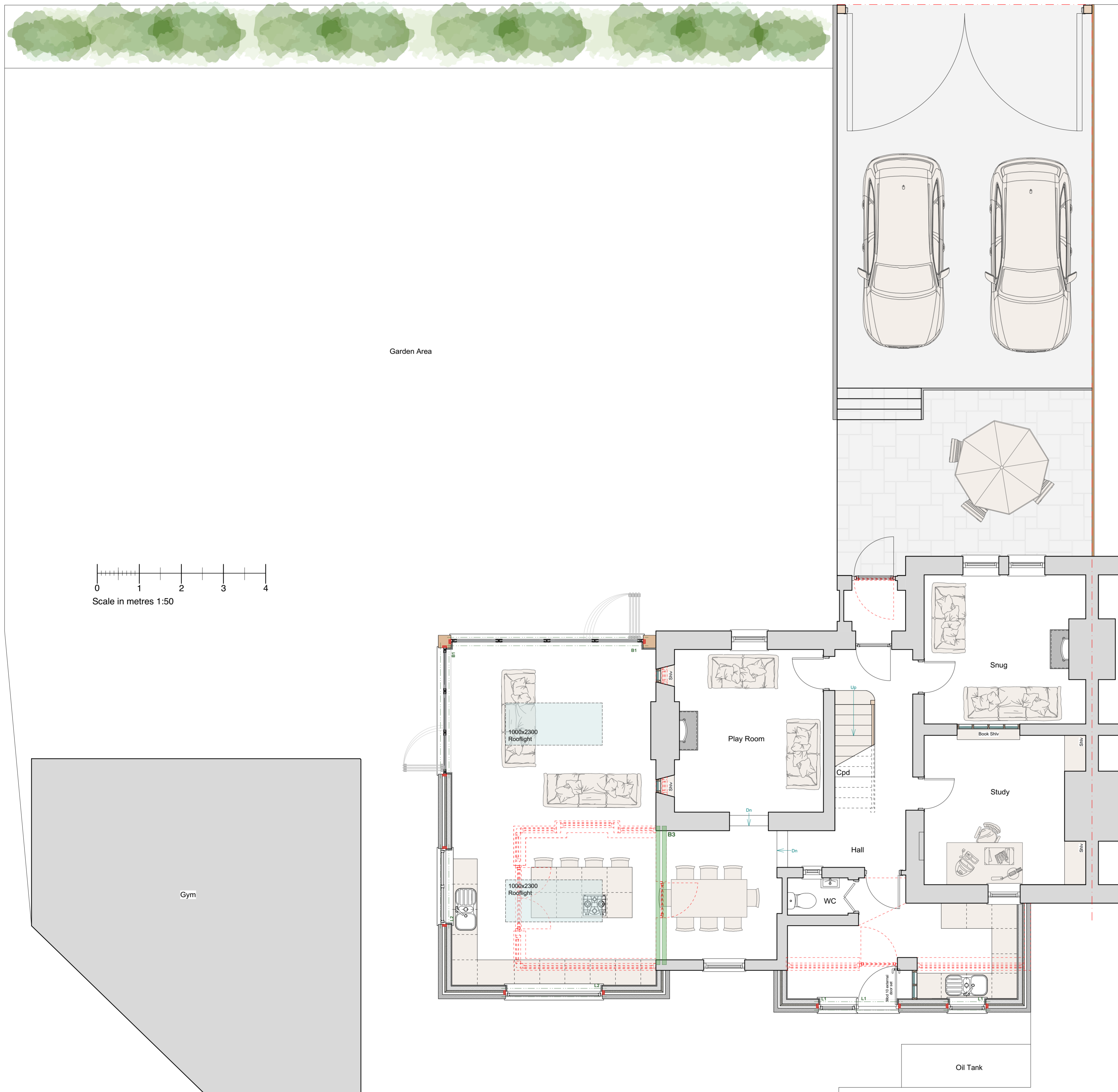
Ground Floor Plan 1:50
