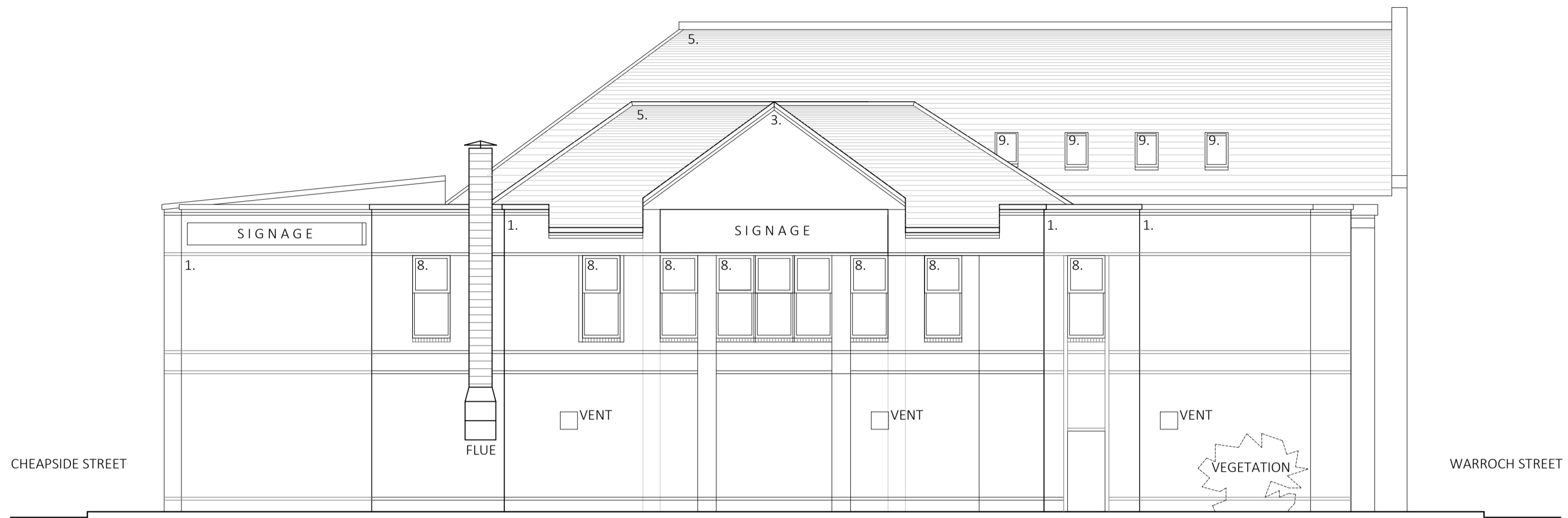
NORTH ELEVATION
