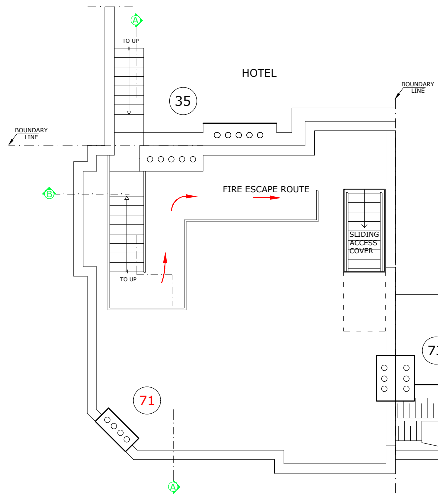
EXISTING ROOF TERRACE PLAN
