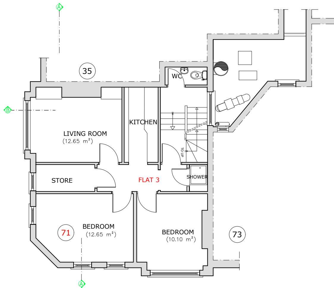
EXISTING THIRD FLOOR PLAN
