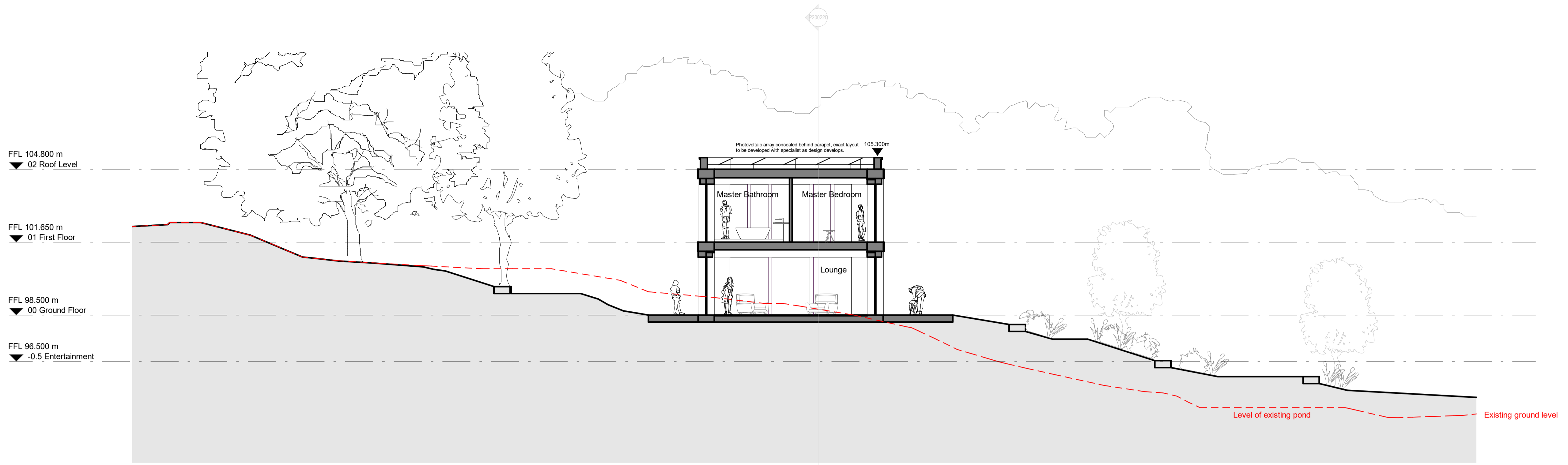
1 PL-Heart House Section, West Facing
