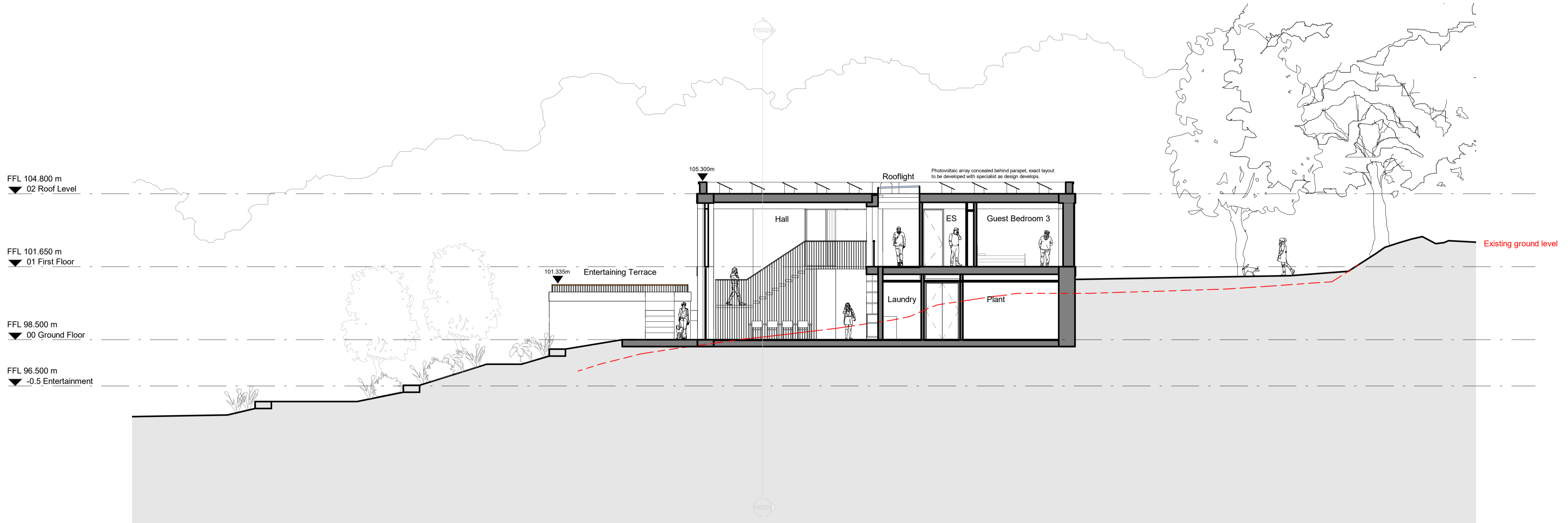
2 PL-Hall Section, East Facing
