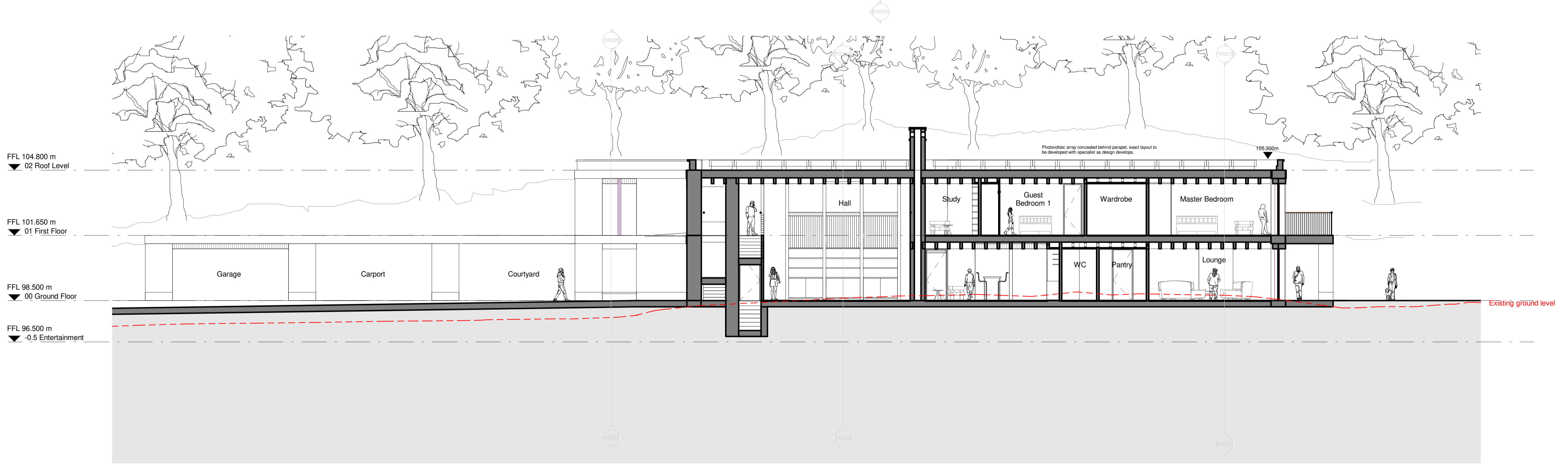
2 PL-Heart House Section, North Facing
