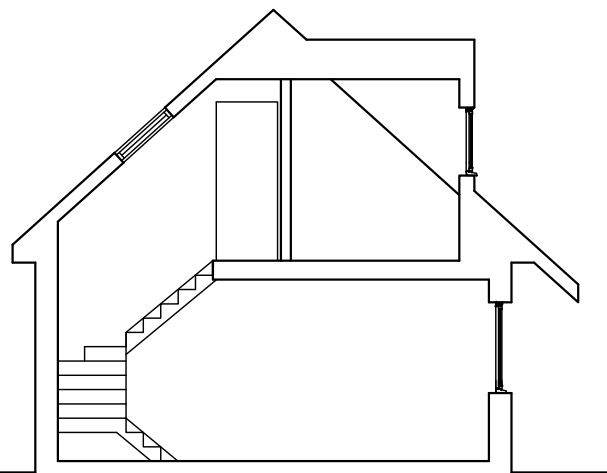
Section through hall
