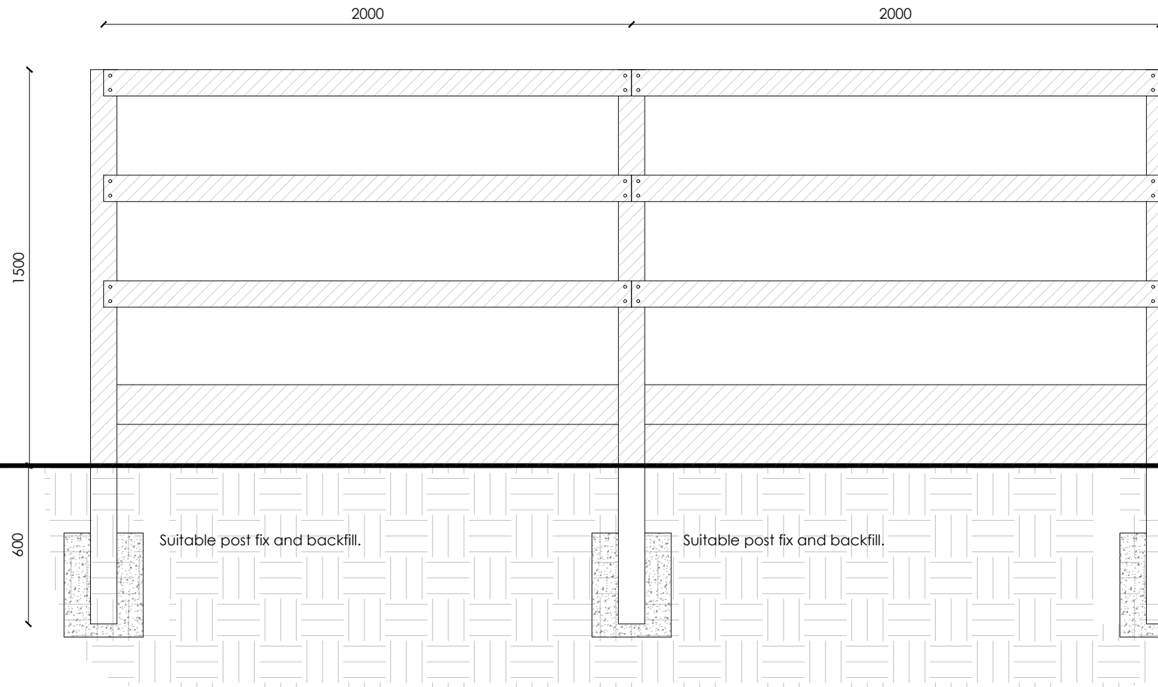
FENCE DETAIL 01
