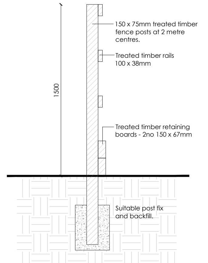
FENCE DETAIL 02
