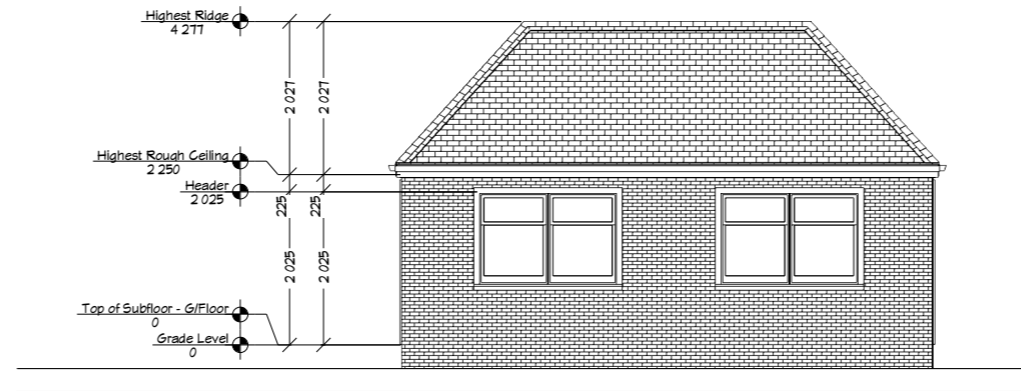
Exterior Elevation Front
