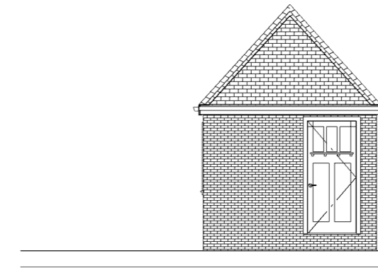
Exterior Elevation Right
