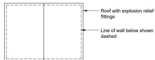
Roof Plan
