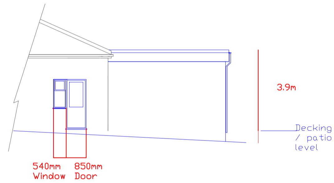
Proposed Right Hand (North) Elevation
