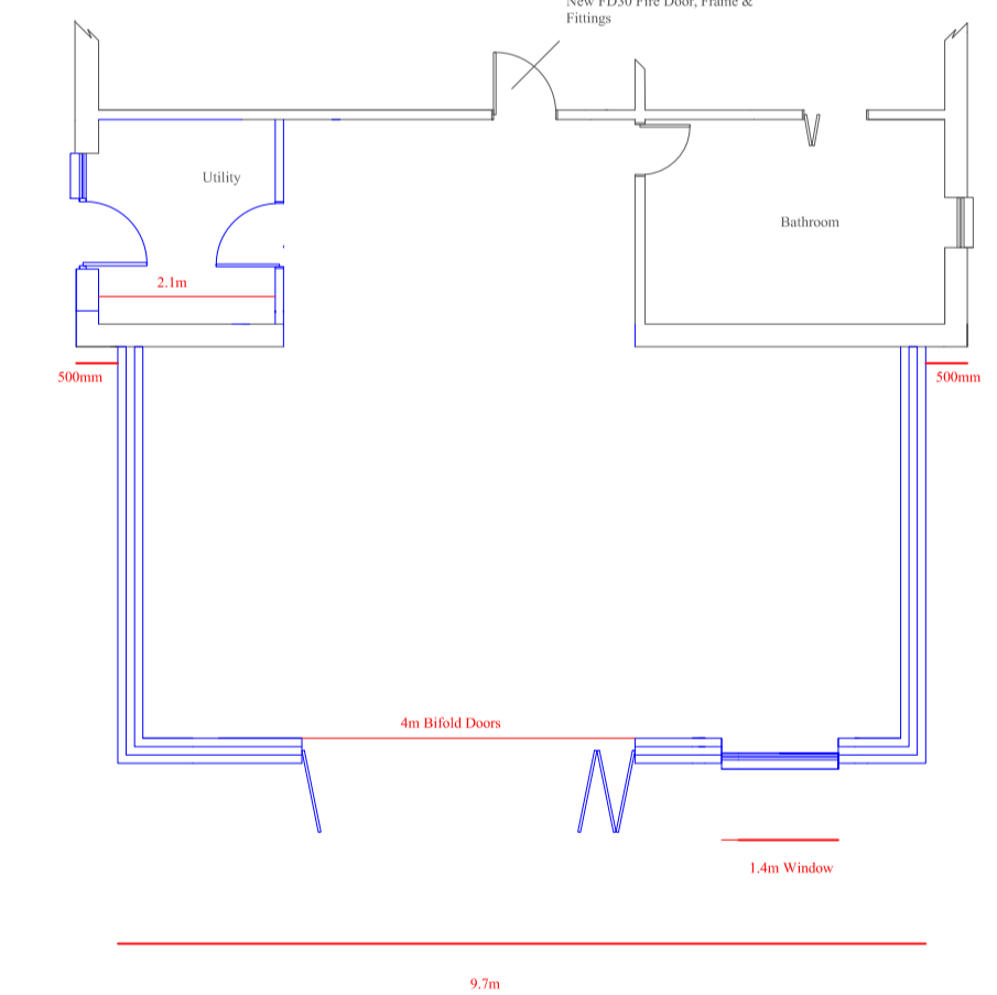
Proposed Floor Plan V3
