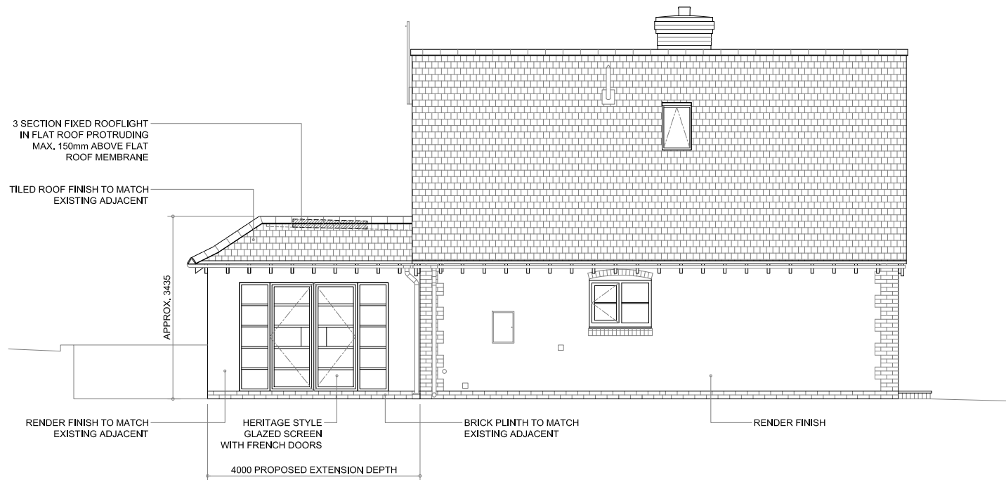
E PROPOSED WEST SIDE ELEVATION SCALE 1:100@A4
