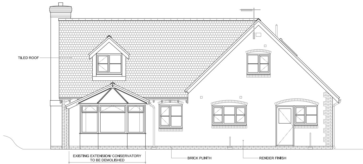
C EXISTING REAR ELEVATION SCALE 1:100@A4
