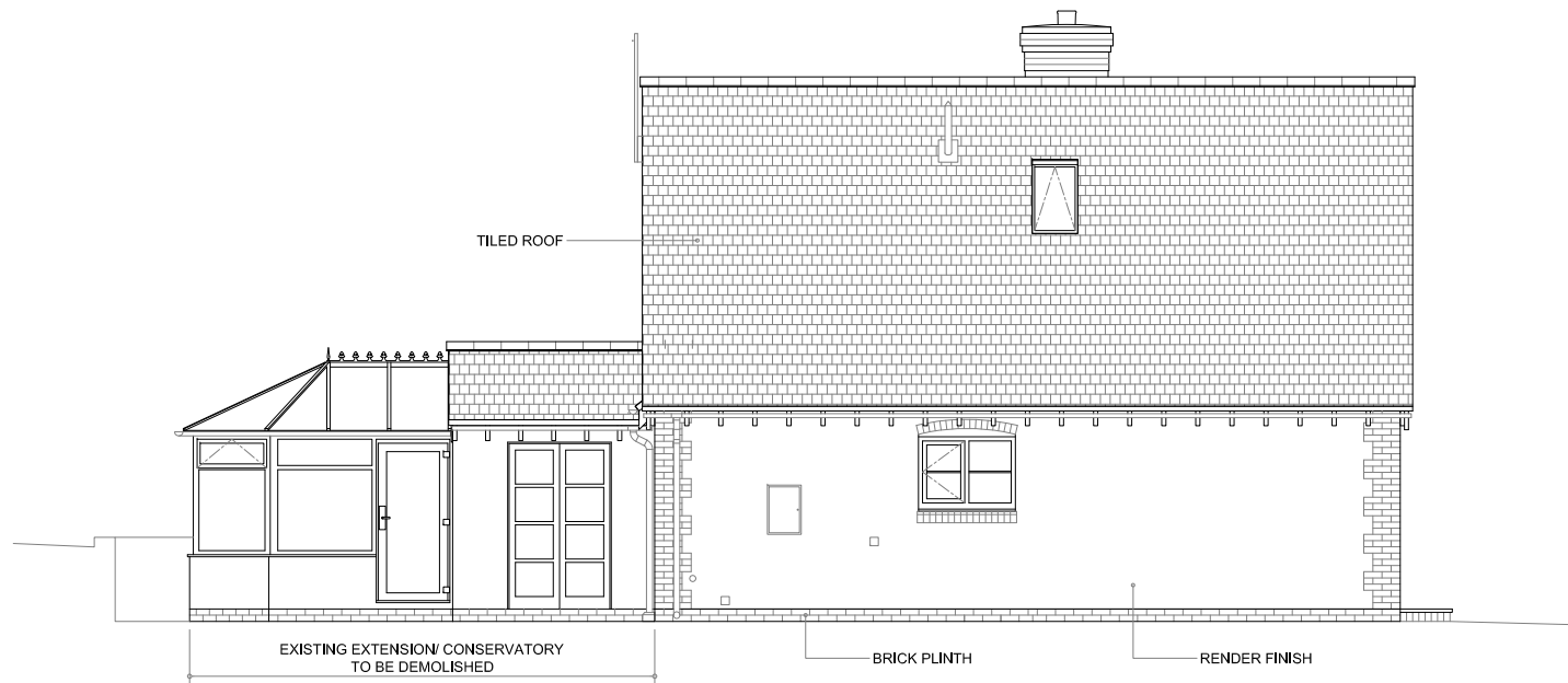
B EXISTING WEST SIDE ELEVATION SCALE 1:100@A4
