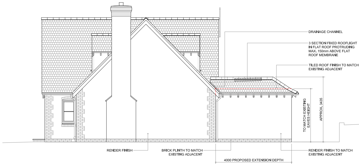
G PROPOSED EAST SIDE ELEVATION SCALE 1:100@A4
