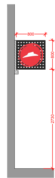
04 SIGNAGE DETAILS 1:50
