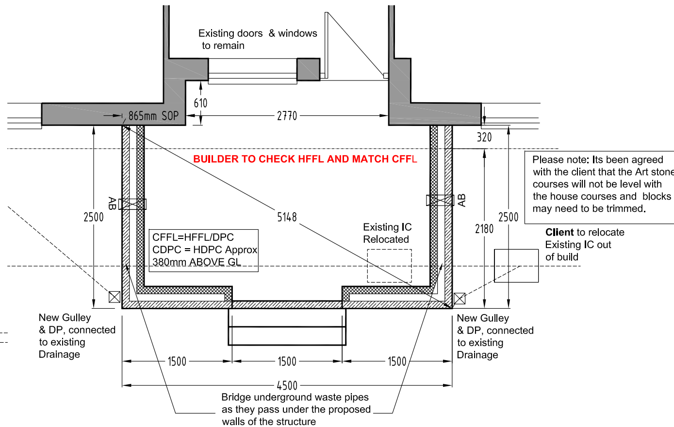
Base Plan - 1:50
