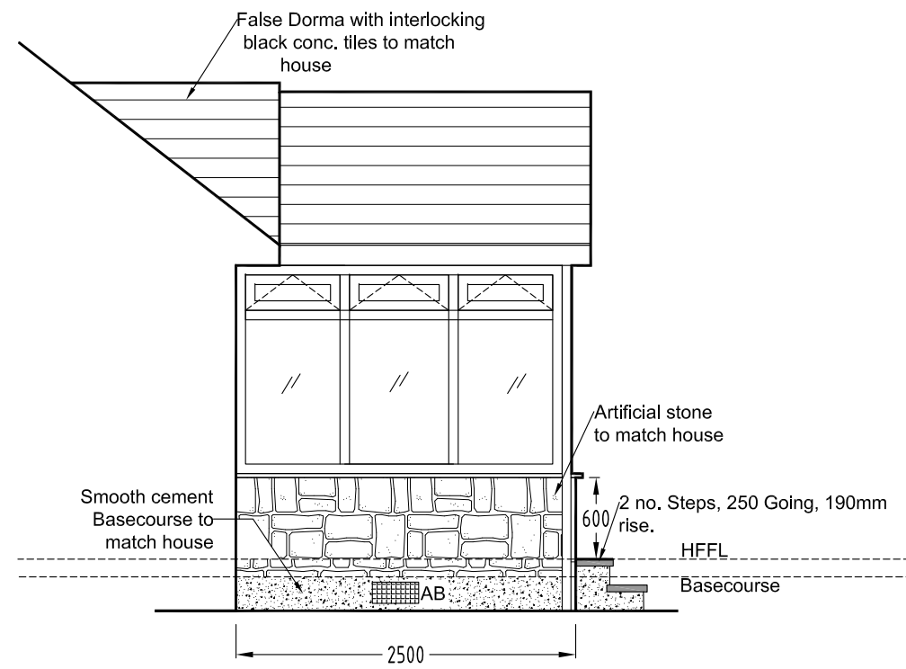
Proposed Left Elevation- 1:50
