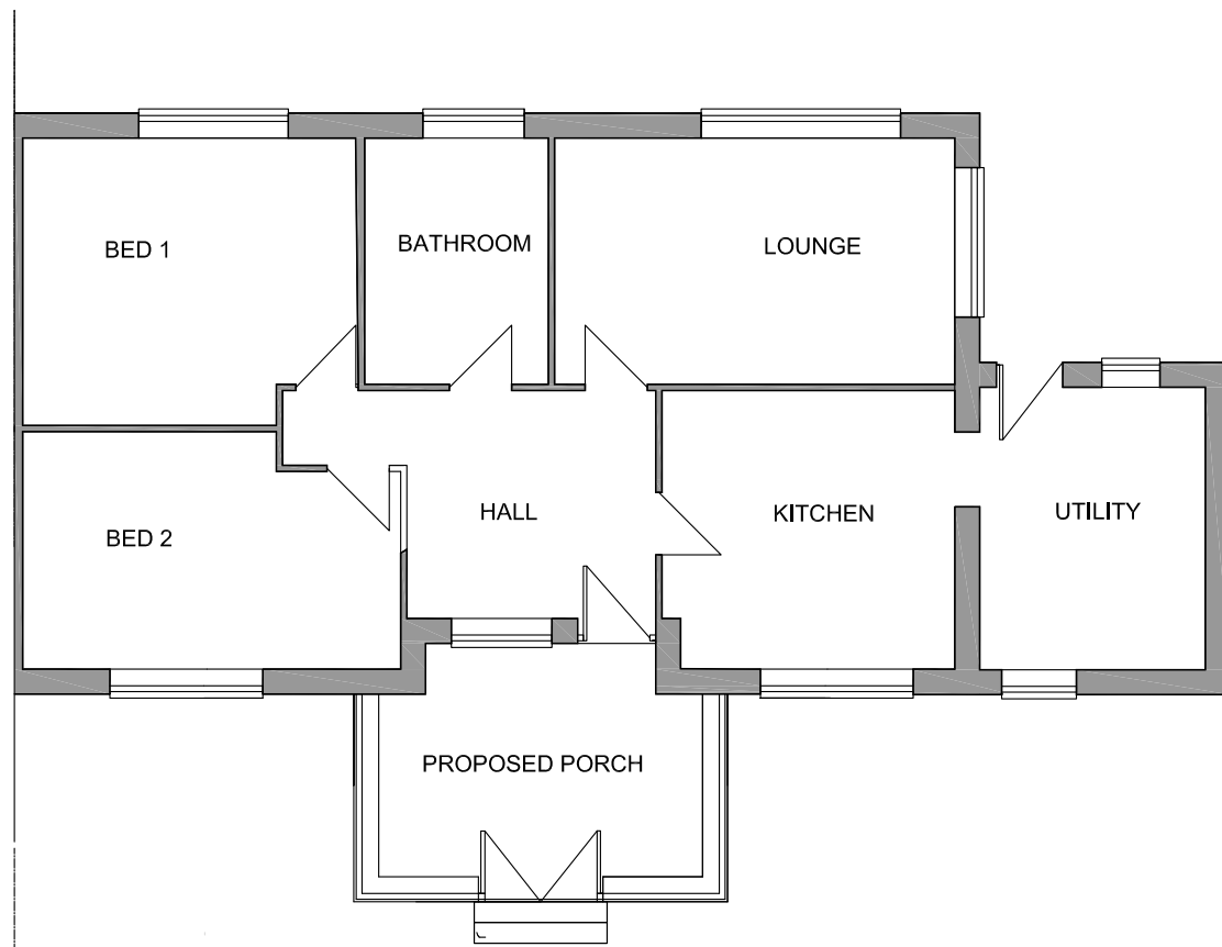
Proposed Floor Plan- 1:100
