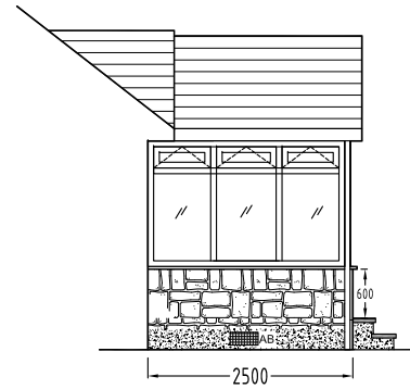
Proposed Left Elevation- 1:100
