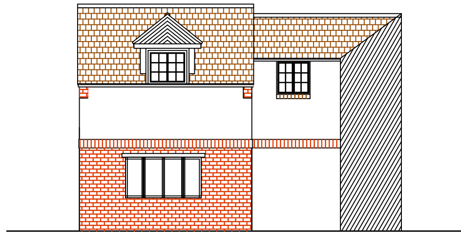
EXISTING SIDE ELEVATION A
