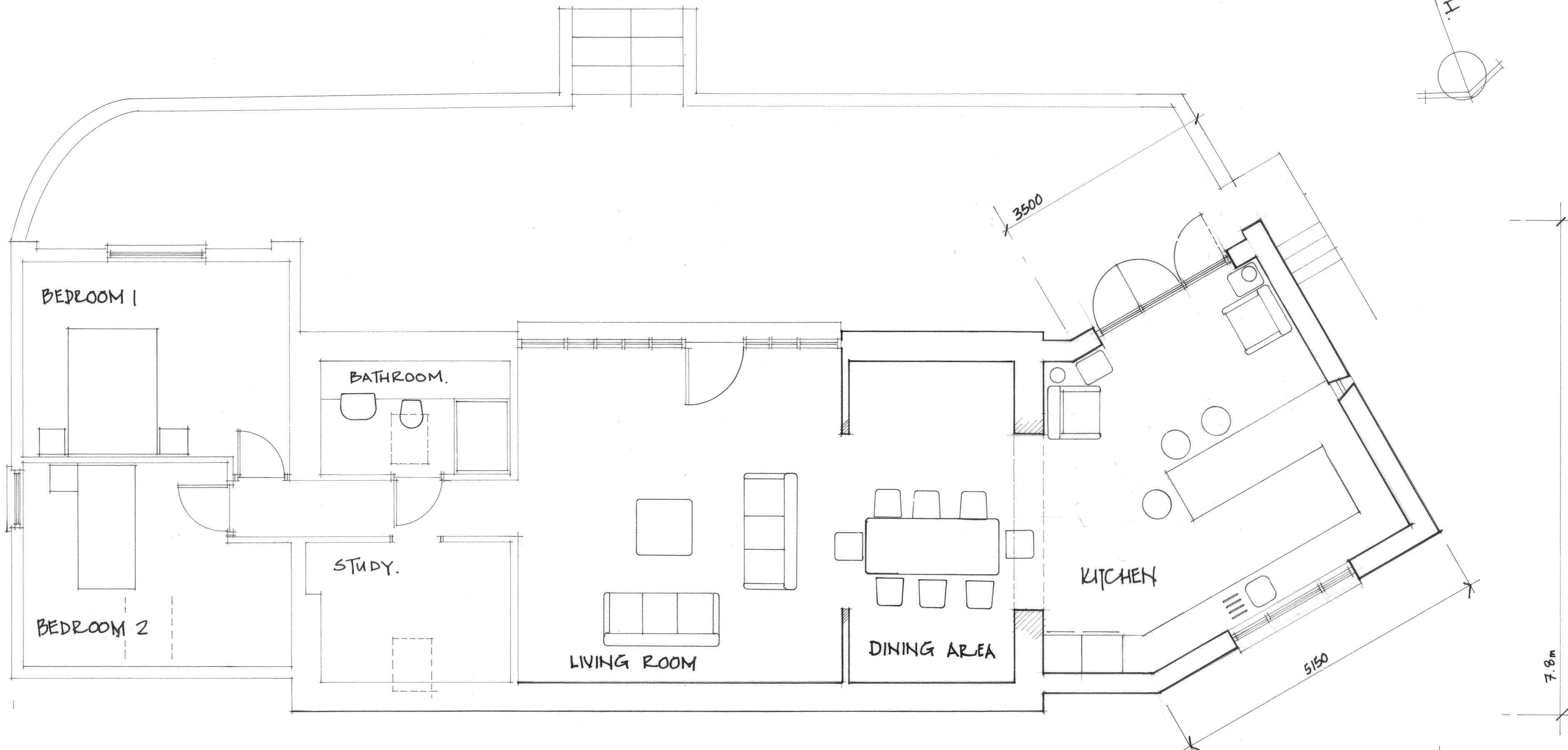
FIRST FLOOR PLAN AS PROPOSED. (1:50)
