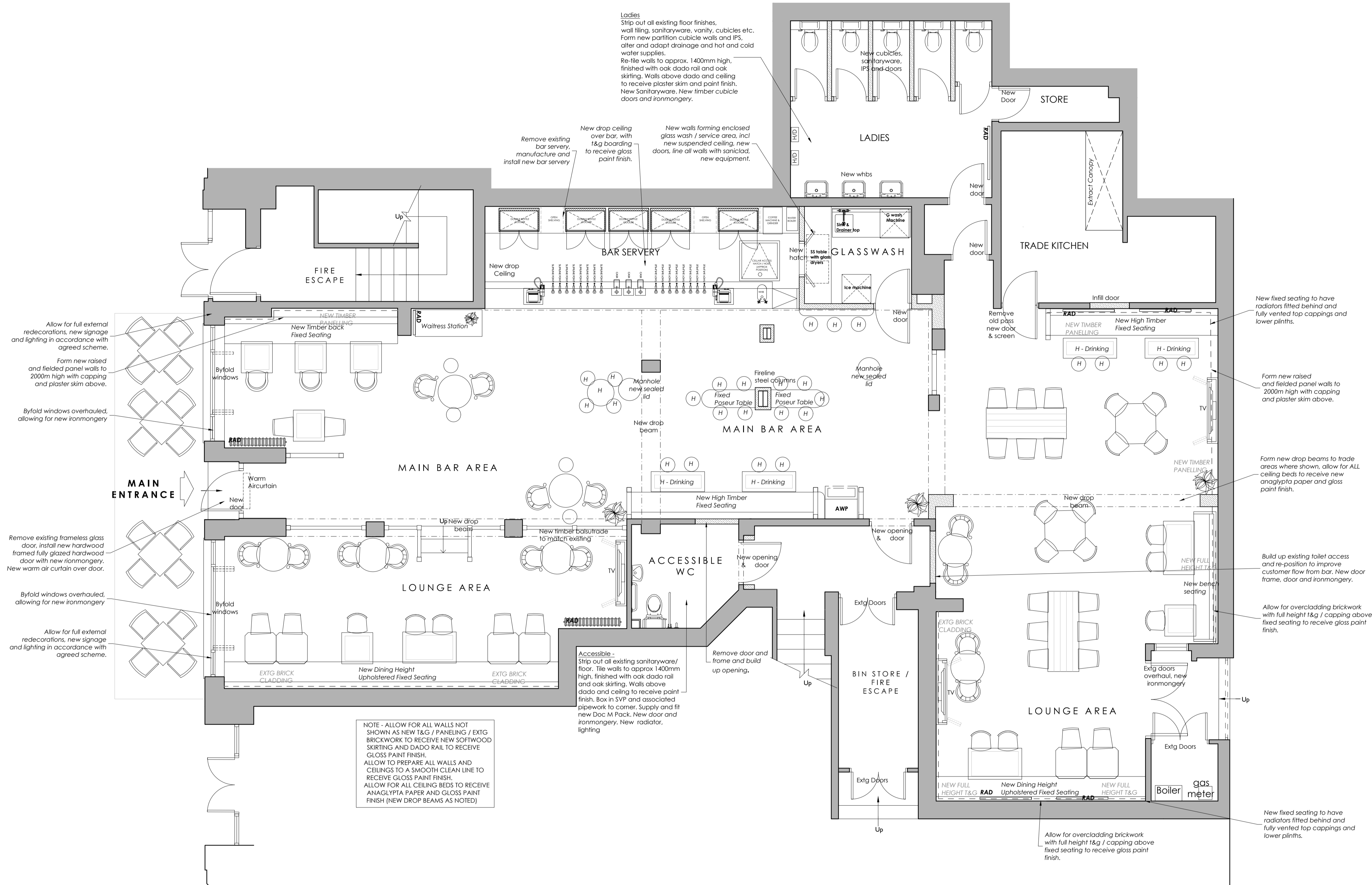
GROUND FLOOR PLAN AS PROPOSED 1:50
