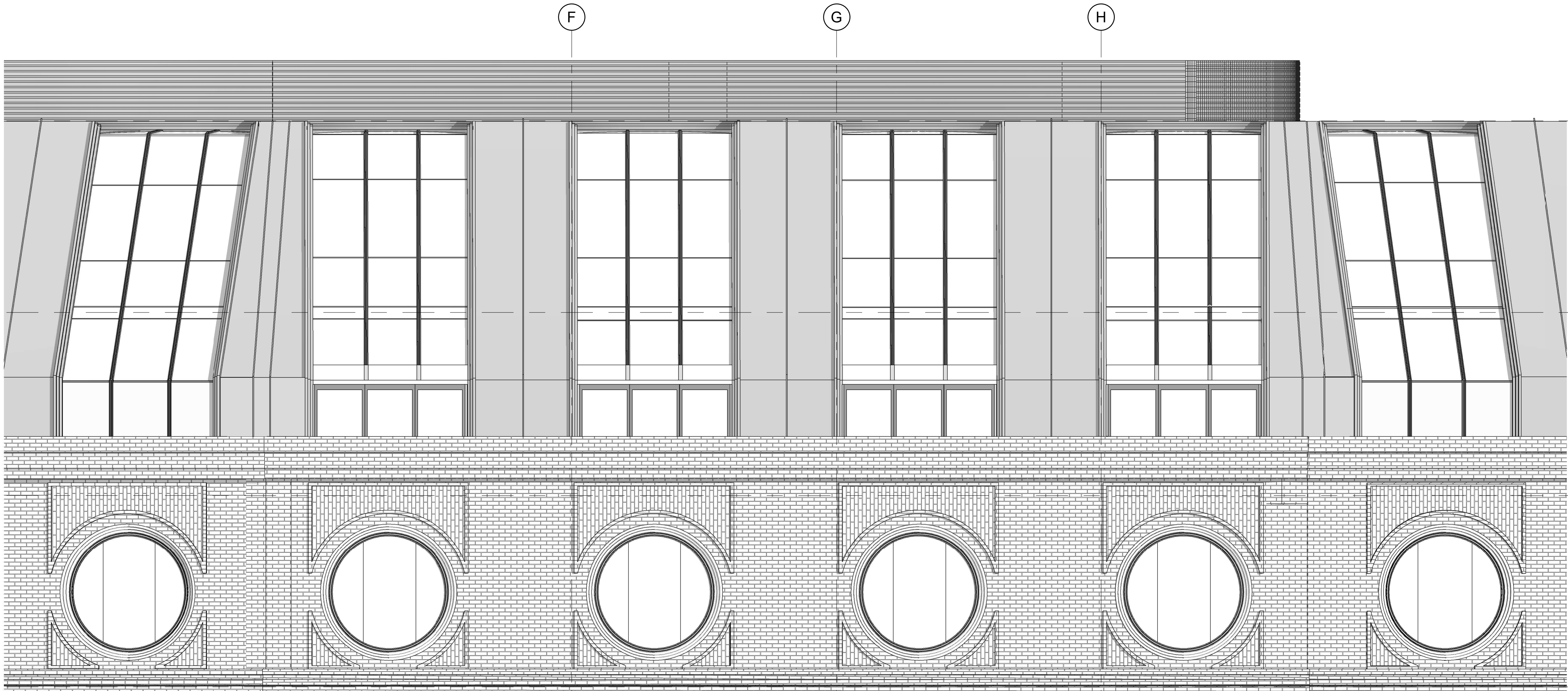
1 Planning 96a - Proposed South Elevation Section 01 PL-P-25-XX-01-12 1 : 50
