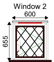
Window 2 1-600x700 White - Gloss 150mm Cill
