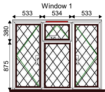
Window 1 1-1600x1300 White - Gloss 150mm Cill
