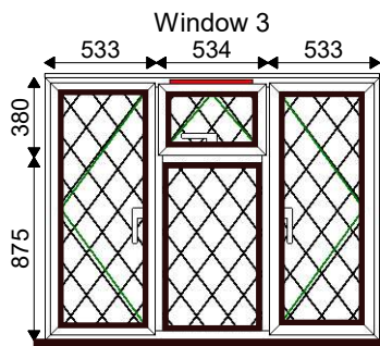
Window 3 1-1600x1300 White - Gloss 150mm Cill
