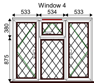
Window 4 1-1600x1300 White - Gloss 150mm Cill
