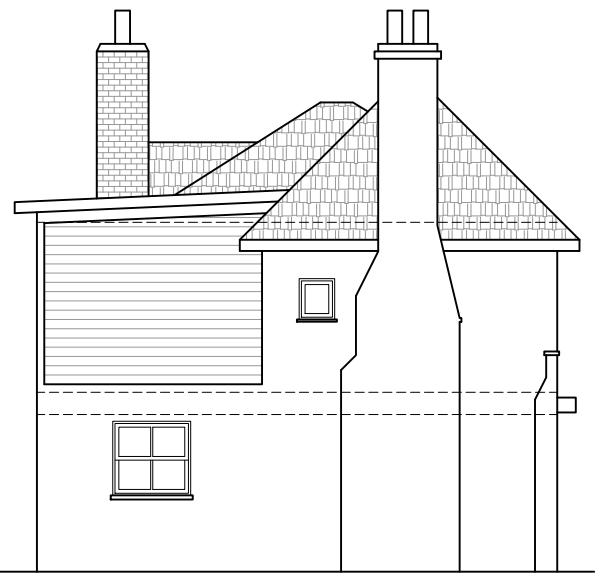
PROPOSED LEFT SIDE ELEVATION
