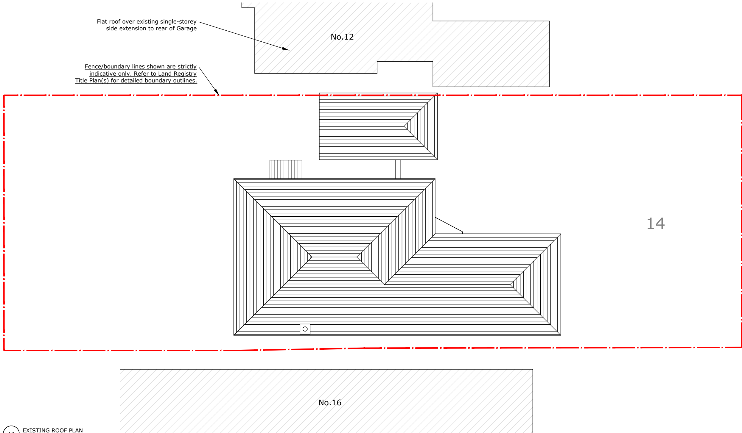
13 EXISTING ROOF PLAN 1:100 @ A3
