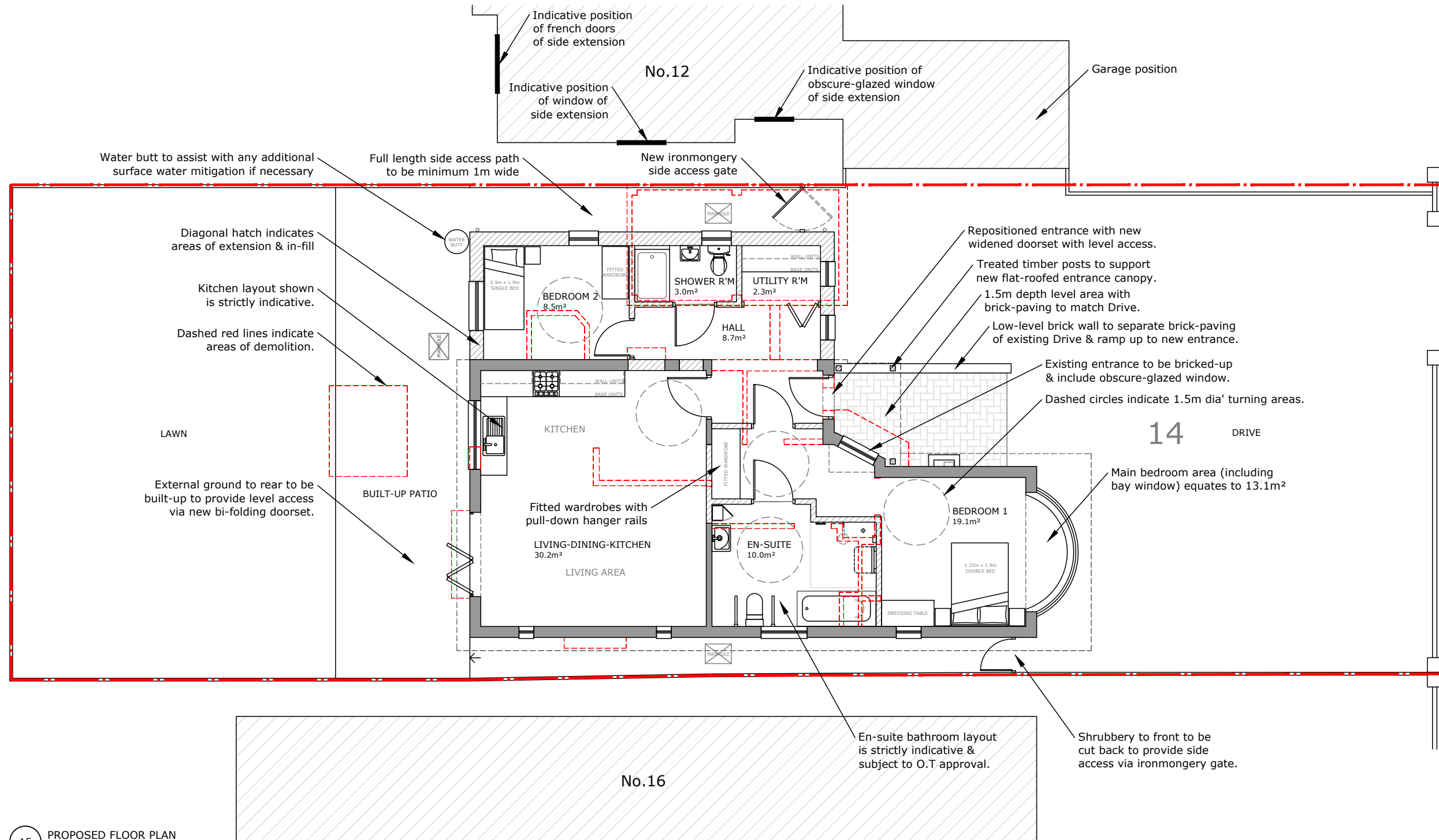
15 PROPOSED FLOOR PLAN 1:100 @ A3
