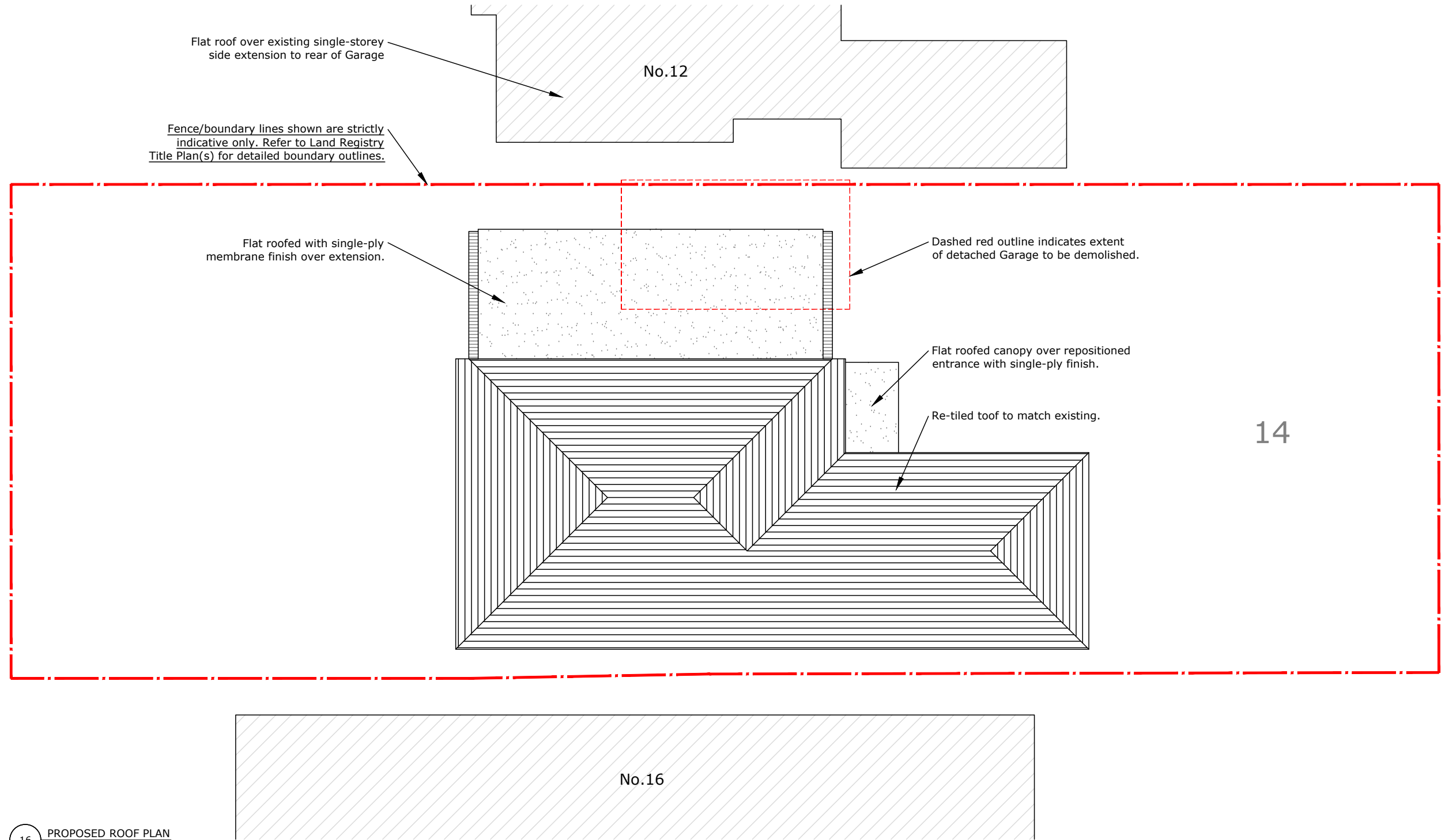
16 PROPOSED ROOF PLAN 1:100 @ A3
