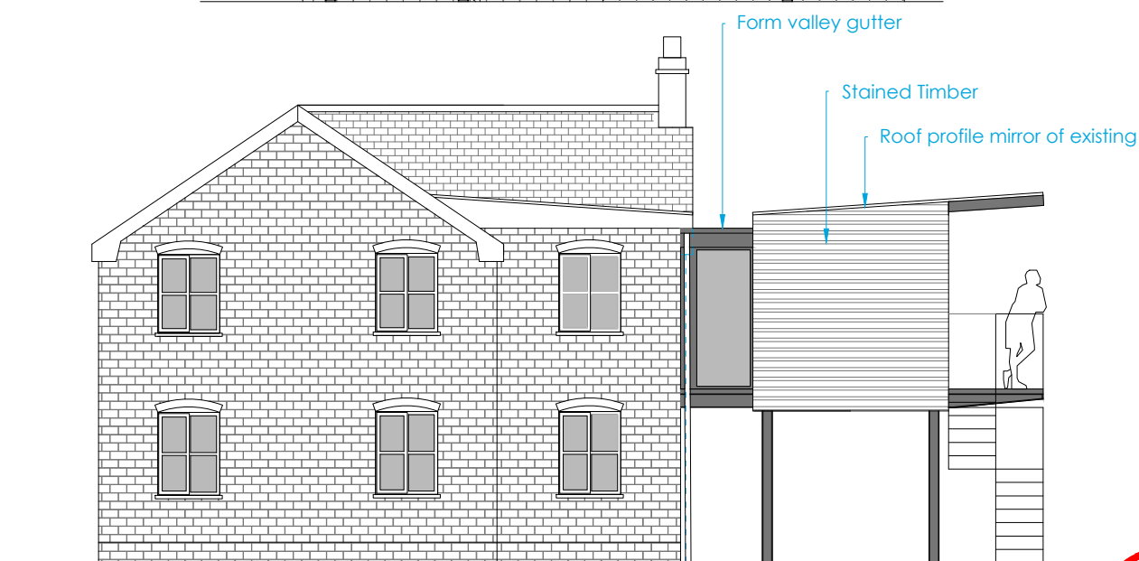
1:100 North Elevation
