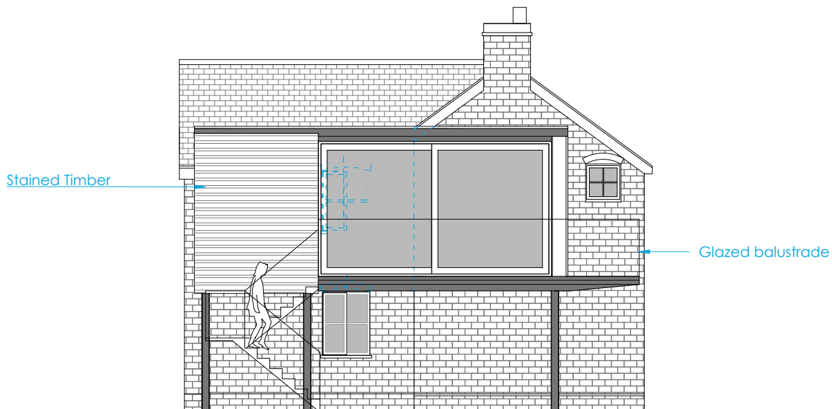
1:100 West Elevation
