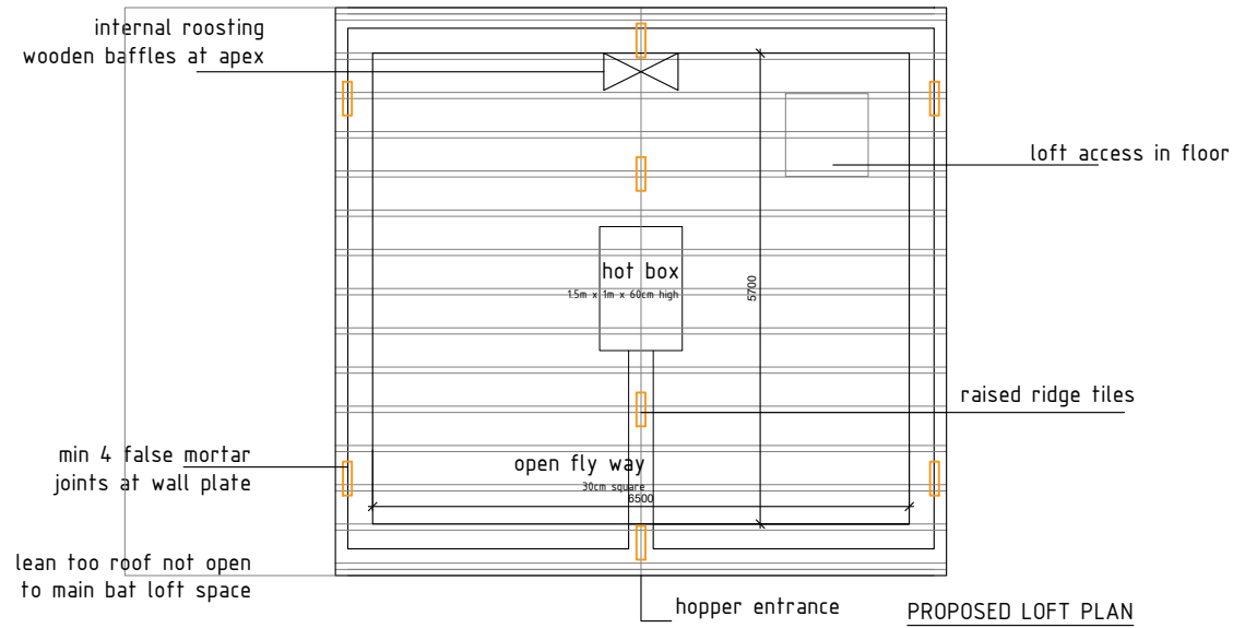
PROPOSED LOFT PLAN
