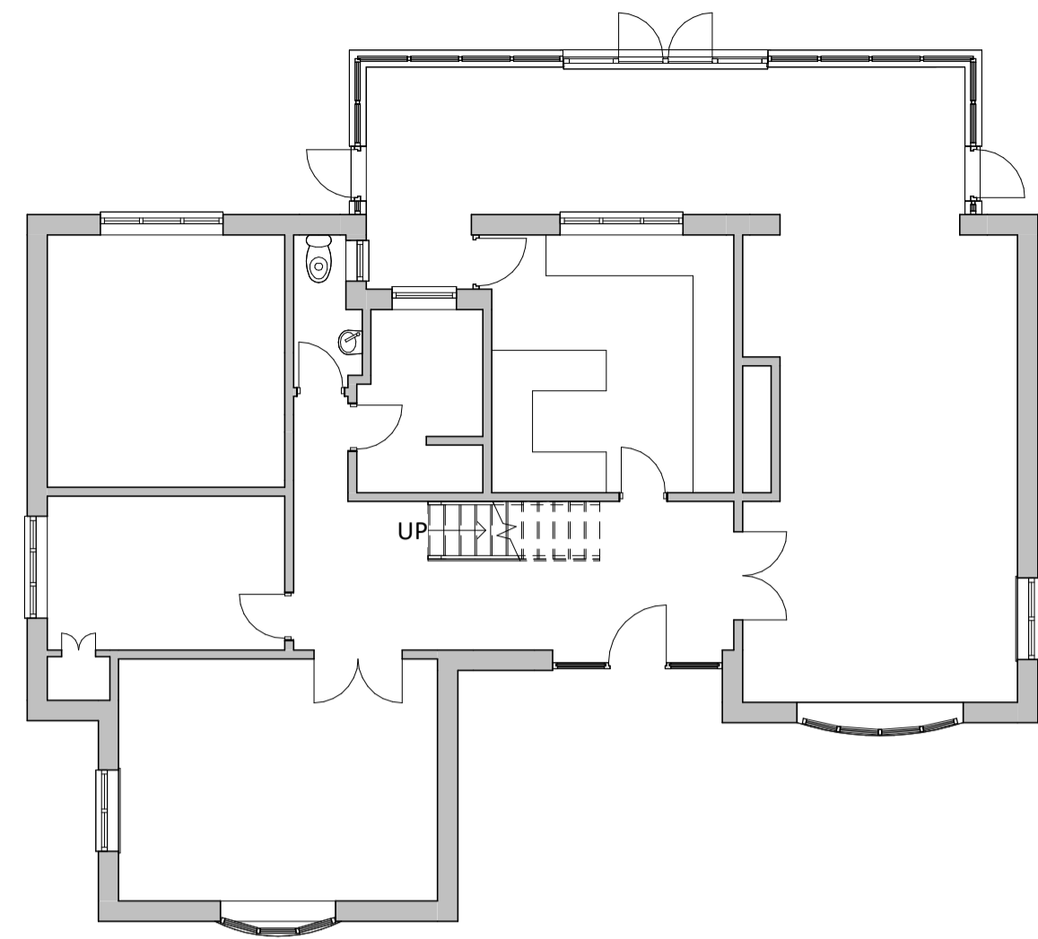
1 Existing Ground Floor Plan 1:100
