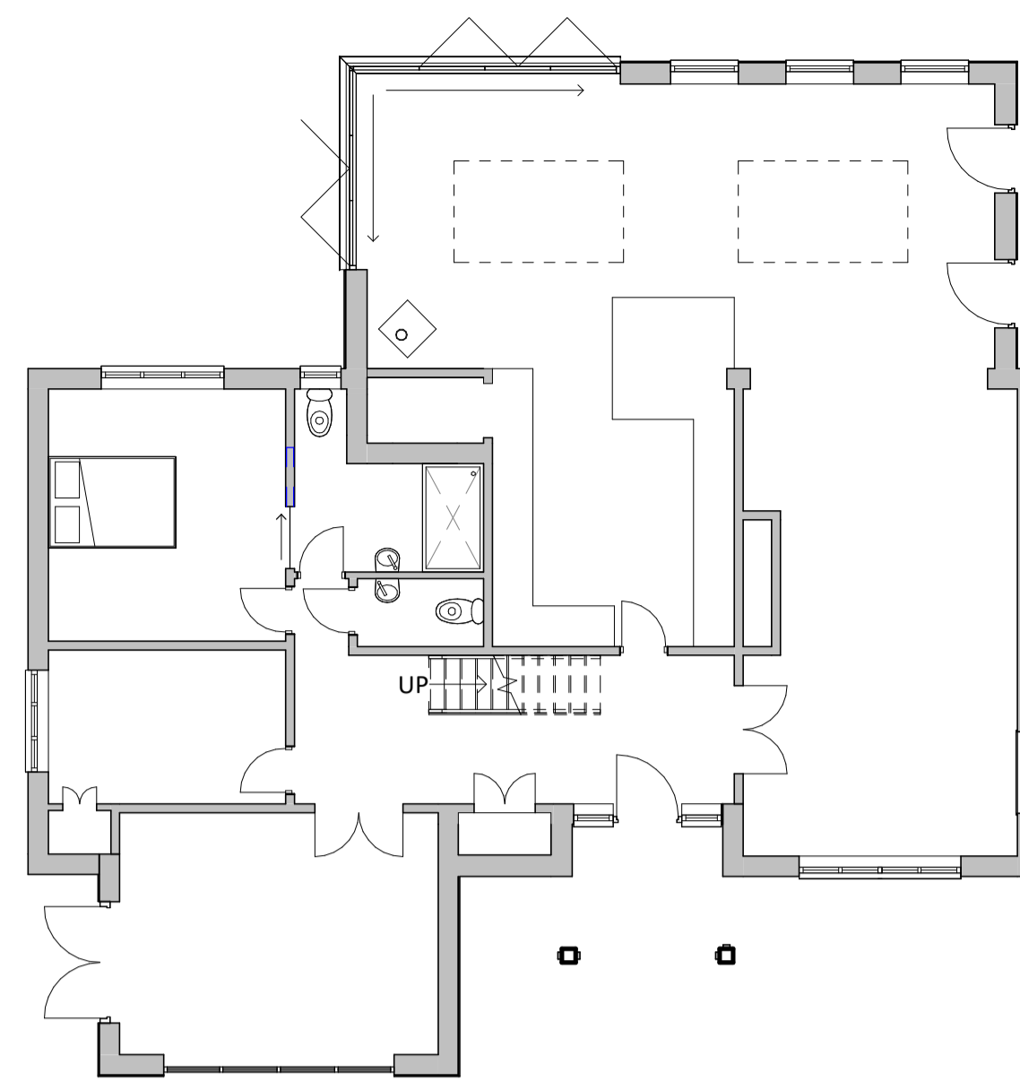
2 Proposed Ground Floor Plan 1:100
