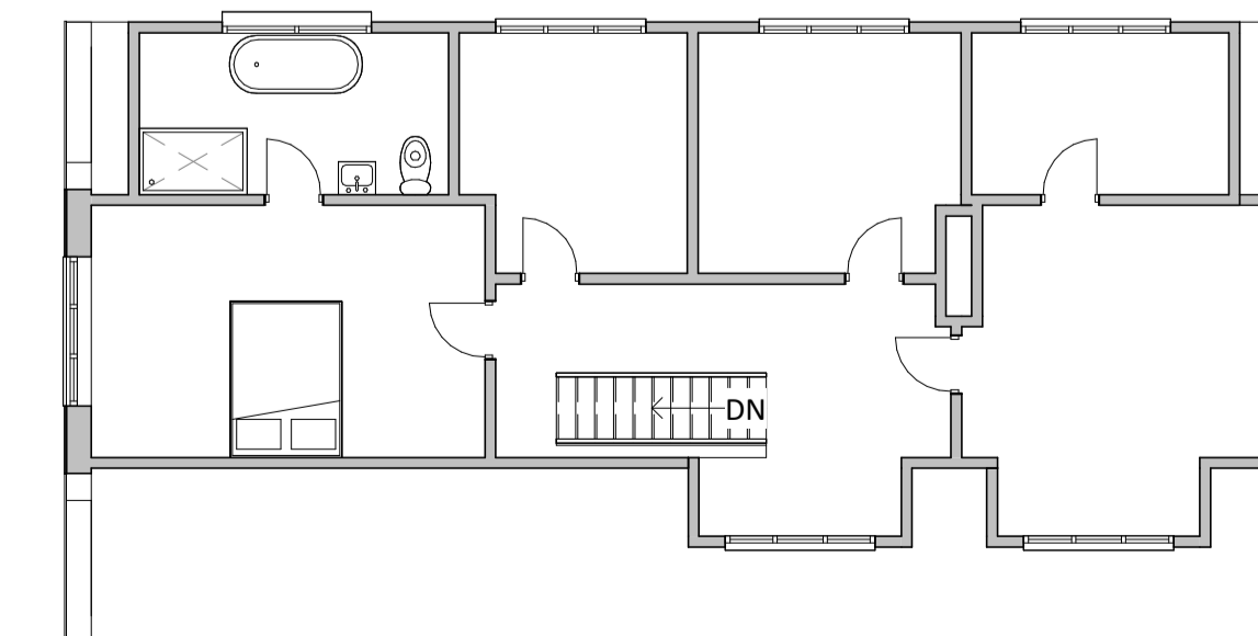
4 Proposed First Floor Plan 1:100
