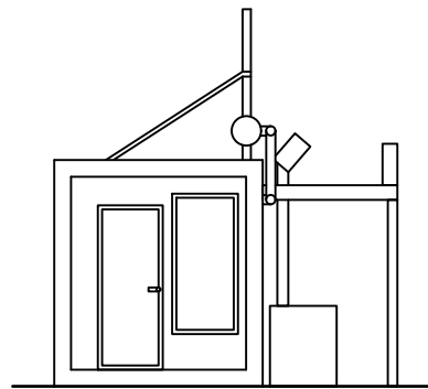
NORTH WEST ELEVATION
