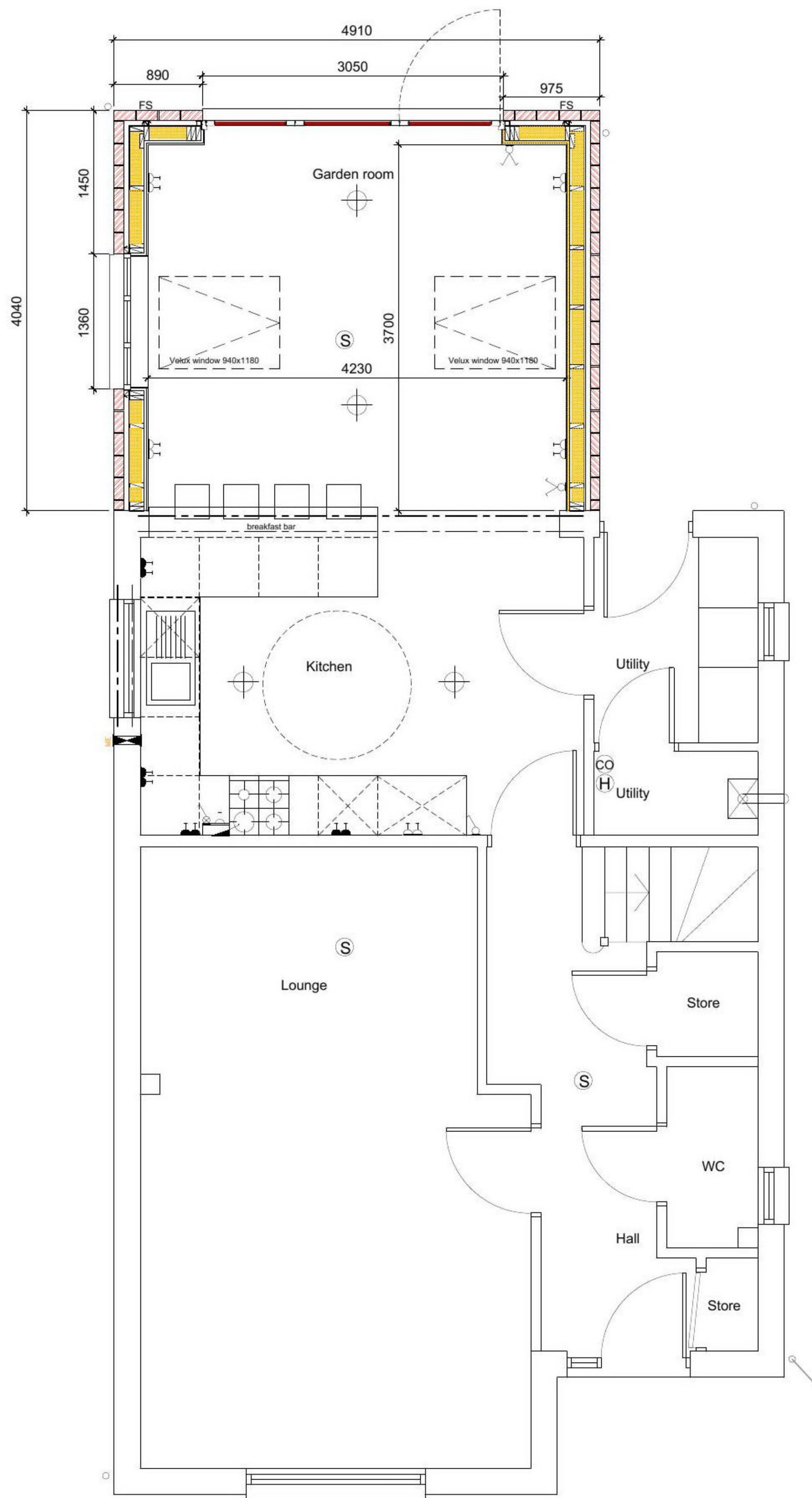
Ground Floor Plan as Proposed
