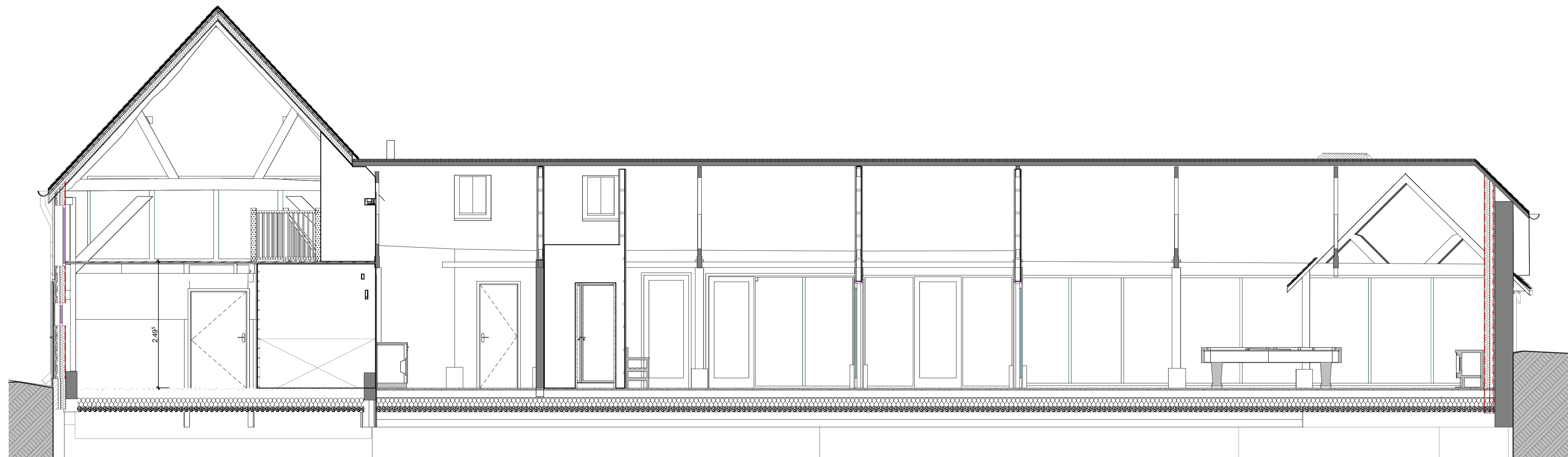
Overall Section D-D 1:50
